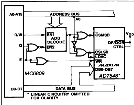
Figure 9. AD7548-MC6809 Interface (Automatic Transfer Mode)
