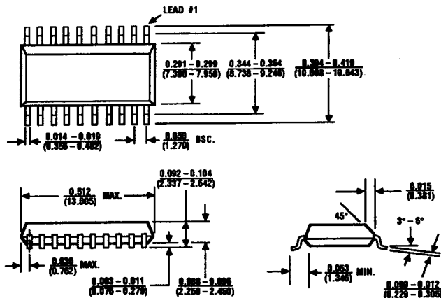
20 Lead Small Outline, Wide (WP)
