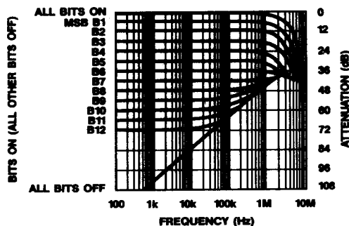
MULTIPLYING MODE FREQUENCY RESPONSE vs DIGITAL CODE
