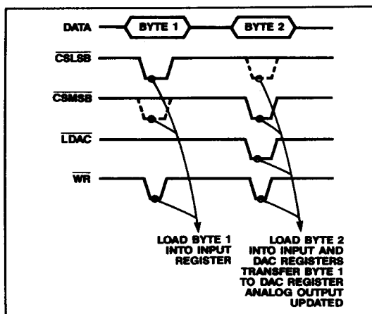
Figure 3. Automatic Transfer Mode
