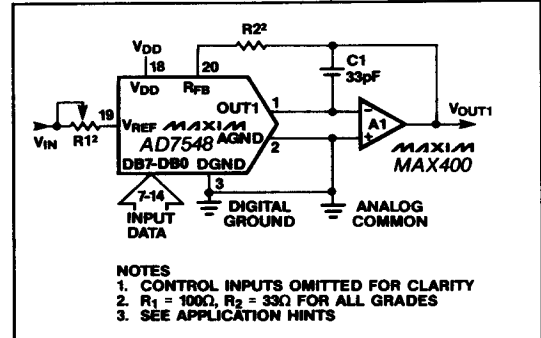
Figure 6. Unipolar Binary Operation
