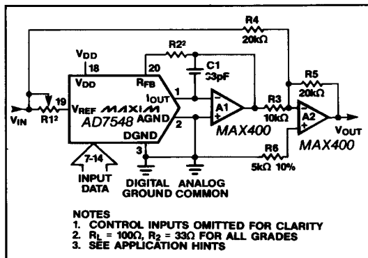
Figure 7. Bipolar Operation (Offset Binary Coding)
