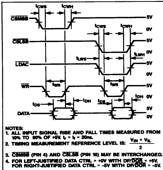
Figure 5. Timing Diagram
