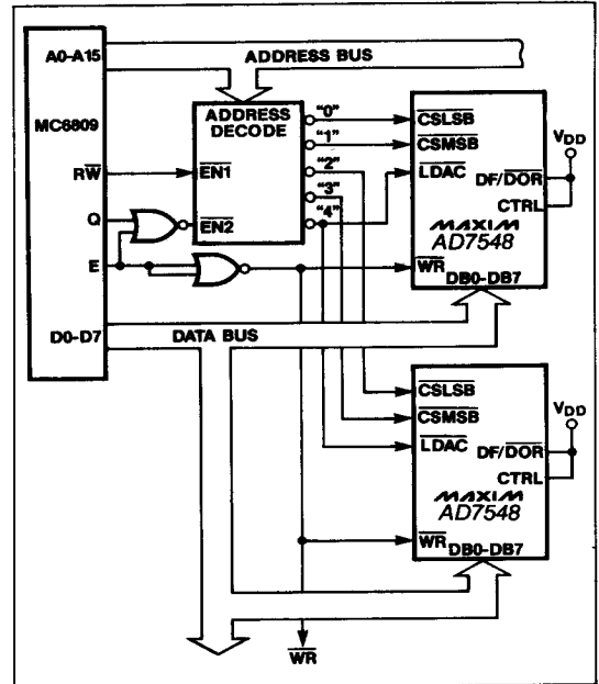
Figure 10. AD7548-MC6809 Interface (Strobed Transfer Mode)
