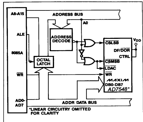
Figure 11. AD7548-8085A Interface (Automatic Transfer Mode)
