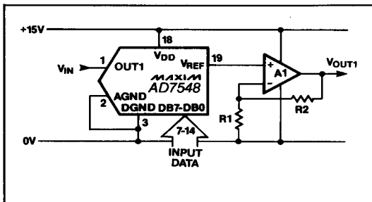
Figure 8. Single Supply Operation Using Voltage Switching Mode
