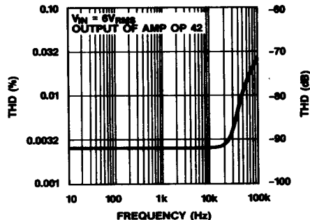
MULTIPLYING MODE TOTAL HARMONIC DISTORTION vs FREQUENCY
