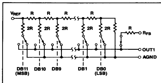
Figure 1. Simplified D/A Circuit of AD7548
