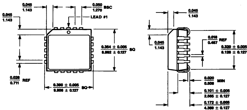
20 Lead Plastic Chip Carrier (Quad Pak) (QP)
