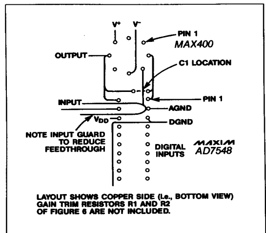
Figure 14. Suggested Layout for AD7548 and Op Amp
