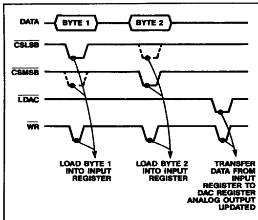
Figure 4. Strobed Transfer Mode
