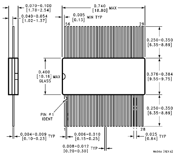
56-Lead Cerpack NS Package Number WA56A
