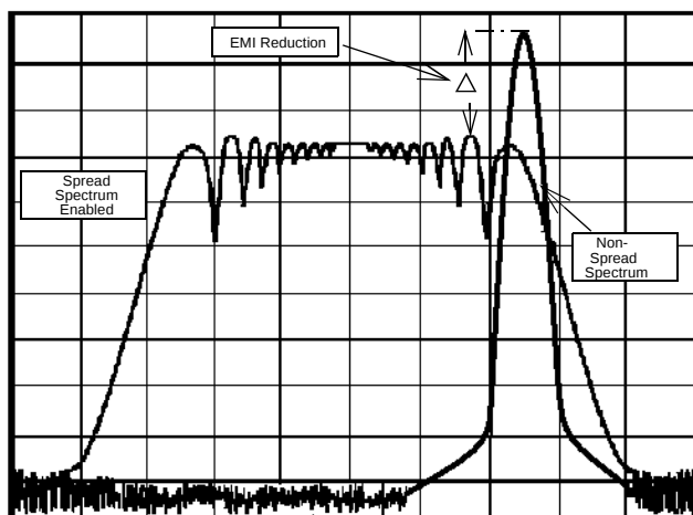
Figure 5. Typical Clock and SSFTG Comparison
