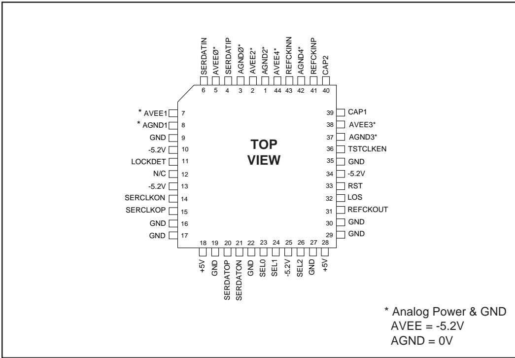
Figure 4. 44 PLCC Pinout
