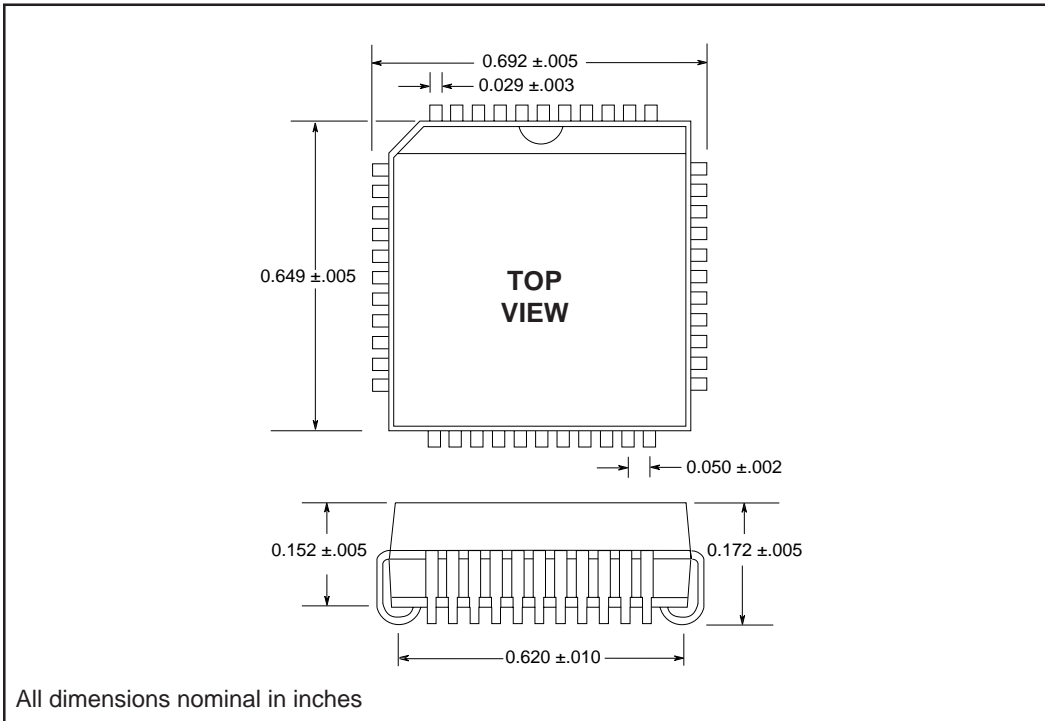
Figure 5. 44 PLCC Package
