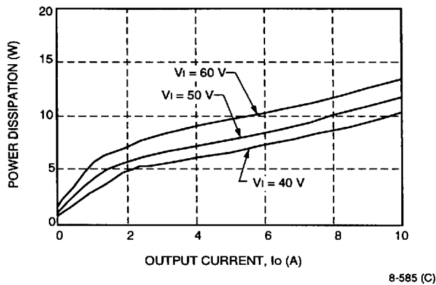
Figure 25. FE050A Power Dissipation as Heat vs. Output Current
