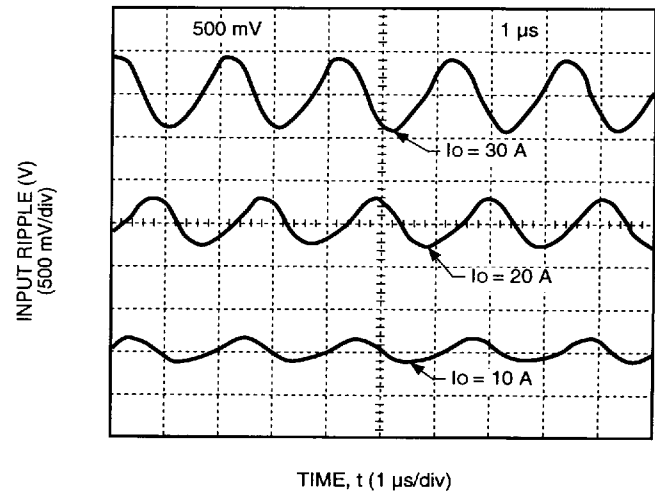
Figure 8. Typical FE150A Input Ripple Voltage at Room Temperature, 48 V Input, and 10 A, 20 A, and 30 A Output
