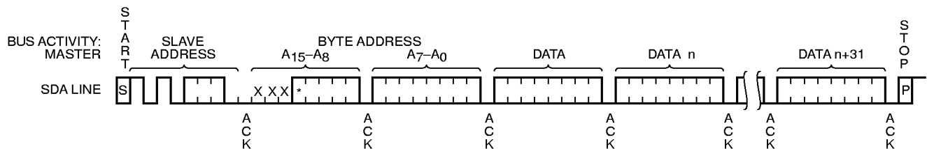
Figure 7. Page Write Timing
