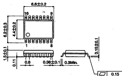
SSOP - A16
