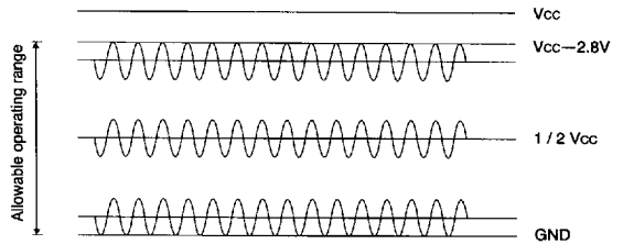
Fig.4 Hall amplifier input bias voltage
