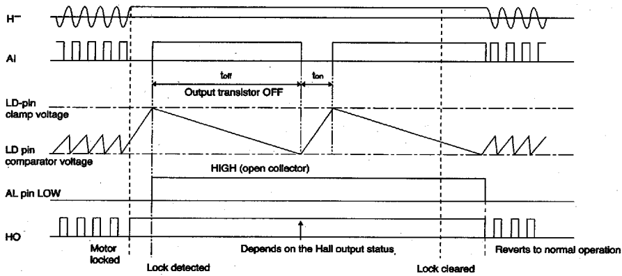
Fig.1 Timing chart for motor locking
