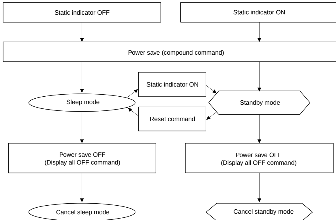
Figure 12-5. Power Save
