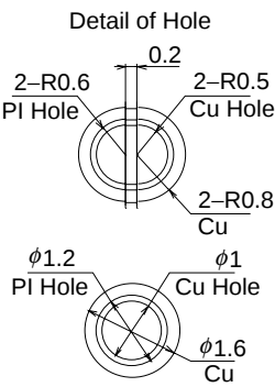
Detail of alignment mark
