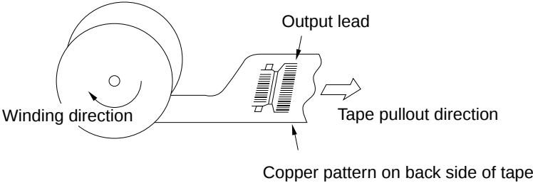
TCP tape winding method
