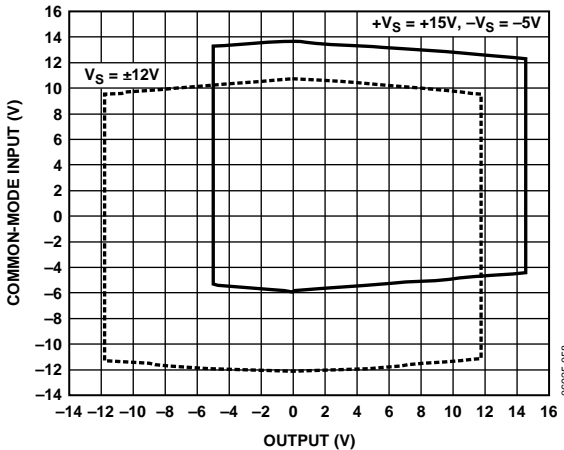
Figure 16. Common-Mode Input vs. Maximum Output Voltage, G = 5 , Large Supplies
