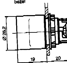
With extended bezel
