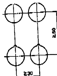
Minimum mounting distances
