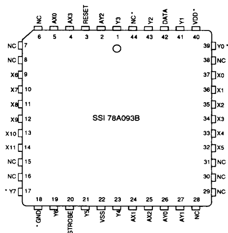
44 - Pin PLCC 78A093B
