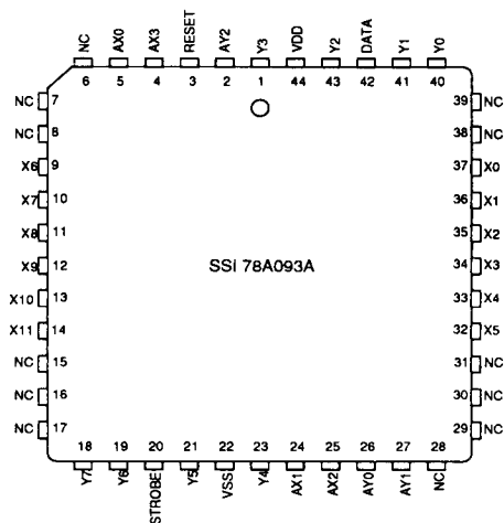
44 - Pin PLCC 78A093A
