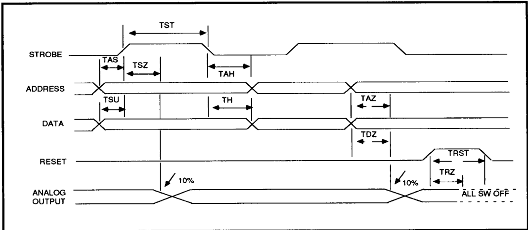
FIGURE 3: Timing Diagram
