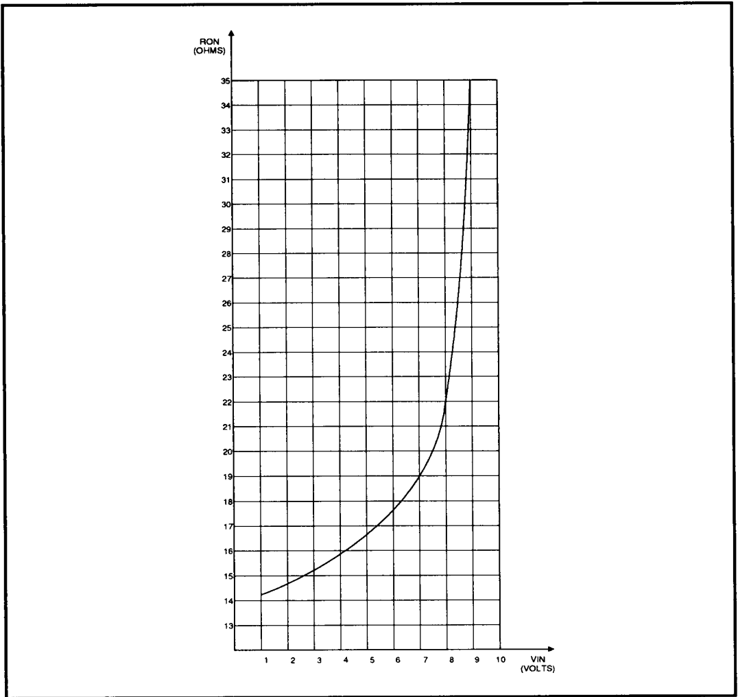
FIGURE 9: X1 - X11 Channel: R_{ON} vs. V_{IN}
