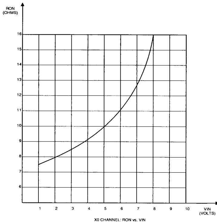
FIGURE 8: X0 - Channel: RON vs. VIN
