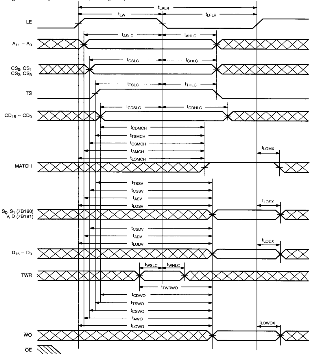
Tag Match Timing in Latch Mode (Showing a Hit)
