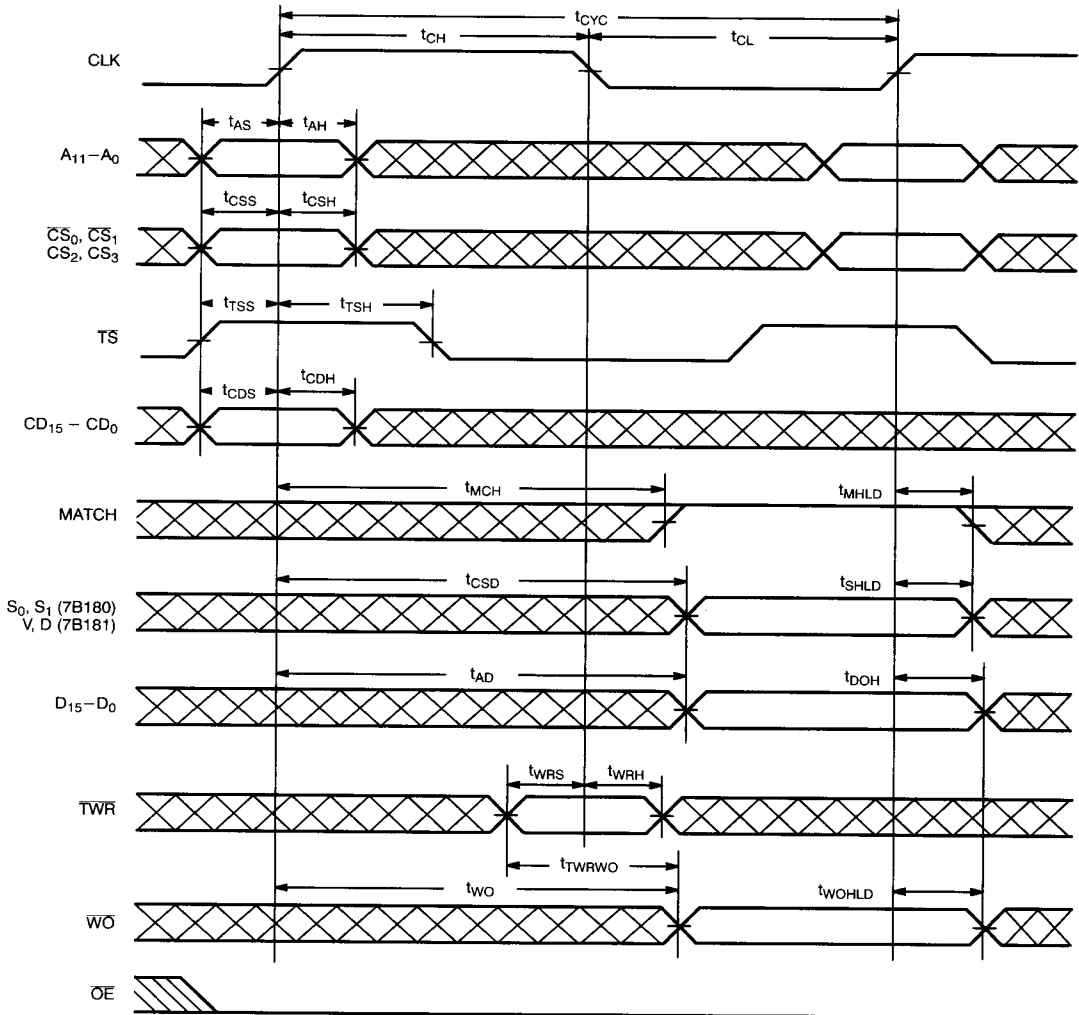
Tag Match Timing in Clock Mode (Showing a Hit)
