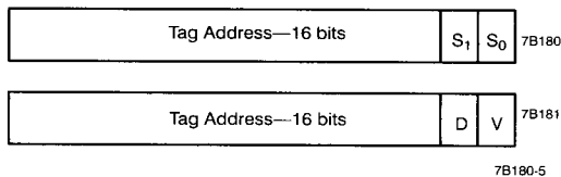
Figure 1. Cache Tag Entry Format
