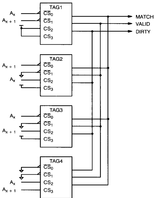
Figure 2. Cascading the CY7B180 and CY7B181
