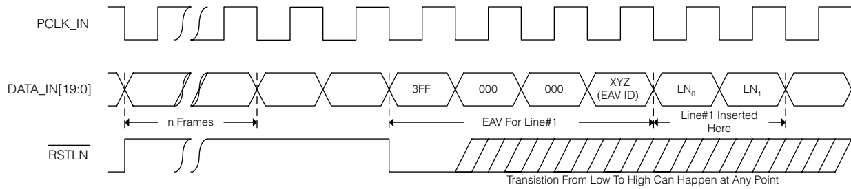
Fig. 2 RSTLN Timing
