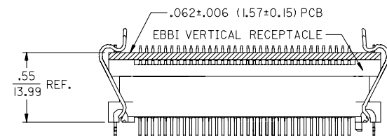
EBBI VERTICAL RECEPTACLE SHOWN LATCHED TO EBBI PLUG (SDA-71660-1***)
