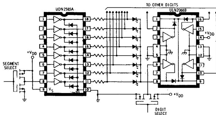
COMMON-CATHODE LED DRIVER
