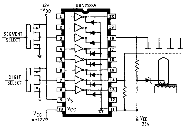
VACUUM-FLUORESCENT DISPLAY DRIVER (Split Supply)
