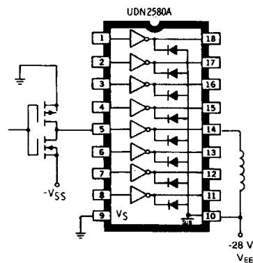
TELECOMMUNICATIONS RELAY DRIVER (Negative Logic)
