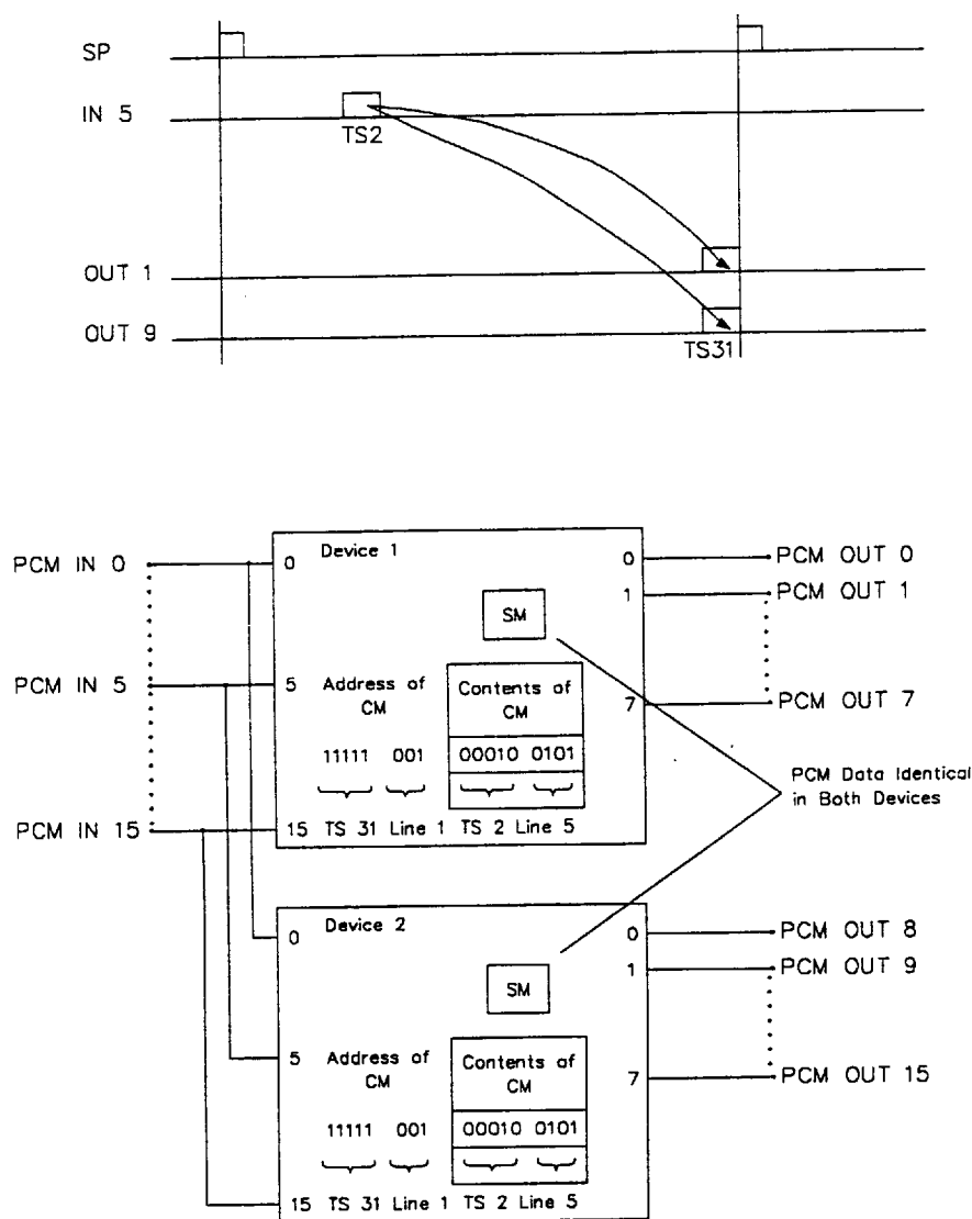
Figure 6.13: Space-time Switch for 512 Subscribers in a 2048 kbps System
