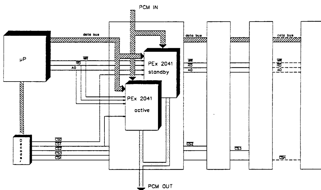
Figure 3.2: Device Setup in Redundant Systems
