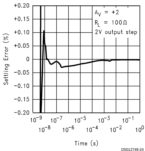
Long-Term Settling Time
