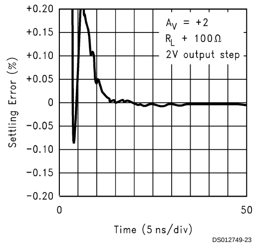
Settling Time
