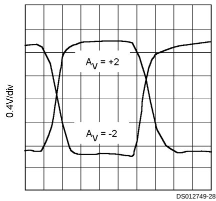
Pulse Response
