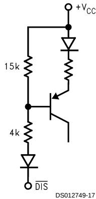
FIGURE 5. Equivalent of (not) DIS input
