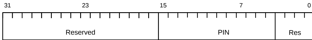
Figure 8. PIO Input Register
