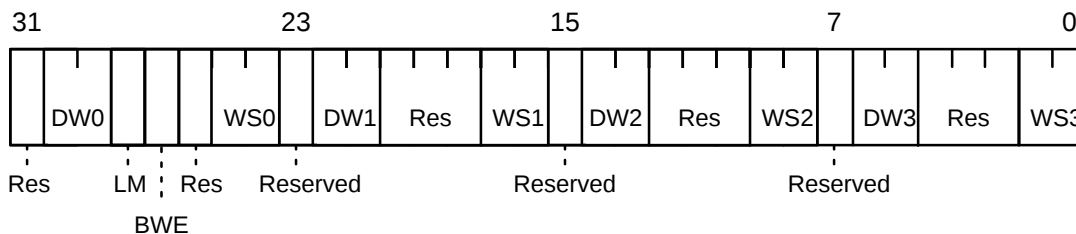
Figure 1. ROM Control Register
