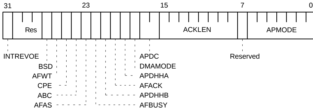
Figure 17. Advanced Parallel Control Register
