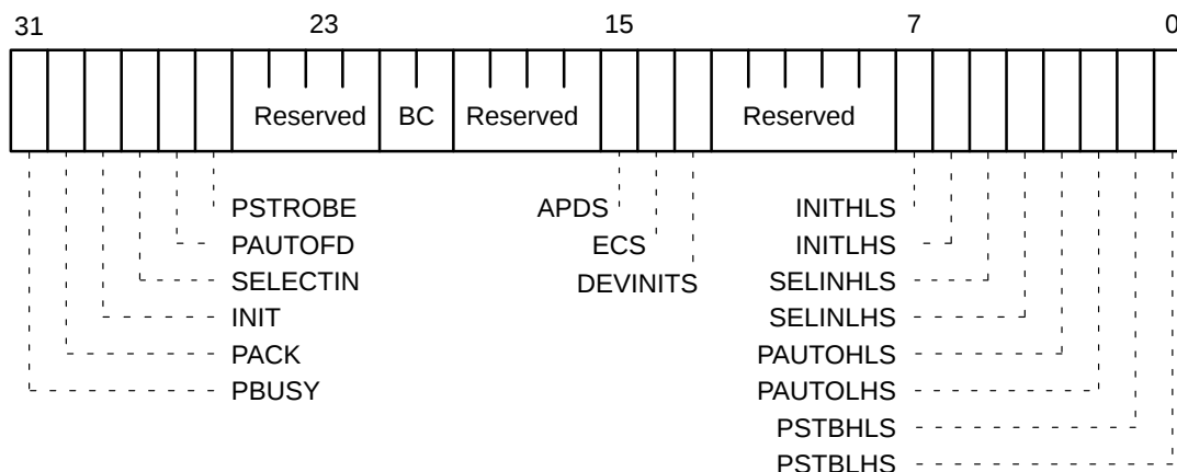
Figure 18. Advanced Parallel Status Register
