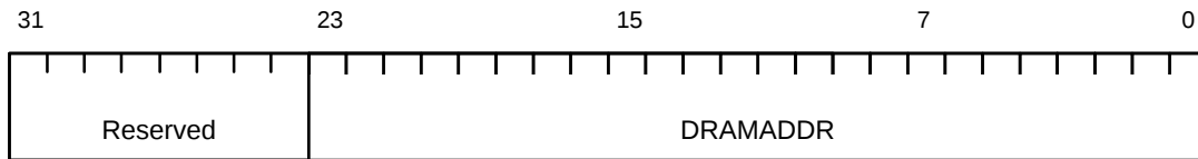
Figure 5. DMA0 Address Register
