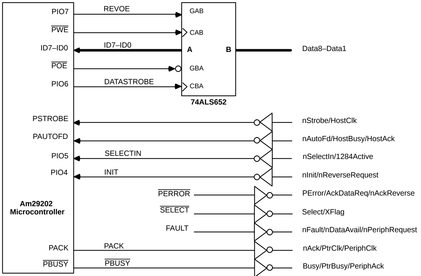
Figure 15. Maximum External System Design
