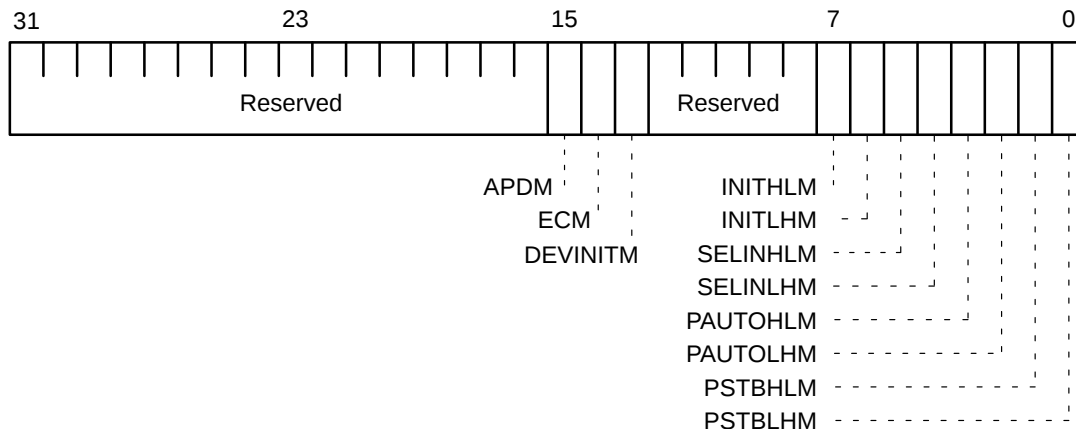
Figure 19. Advanced Parallel Interrupt Mask Register
