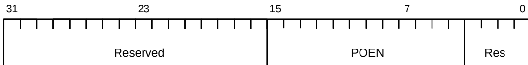
Figure 10. PIO Output Enable Register
