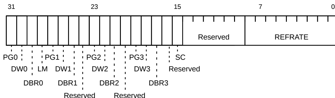
Figure 2. DRAM Control Register
