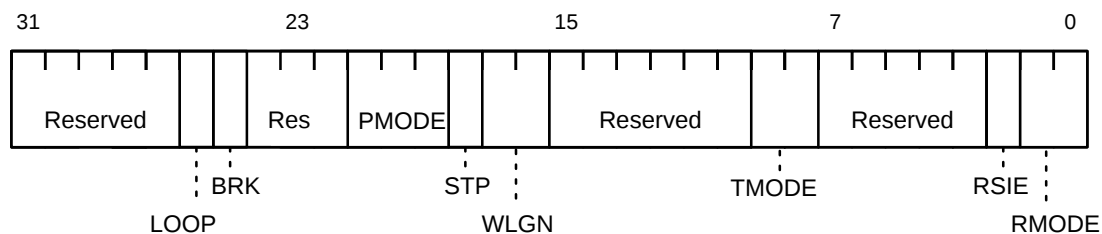
Figure 11. Serial Port Control Register
