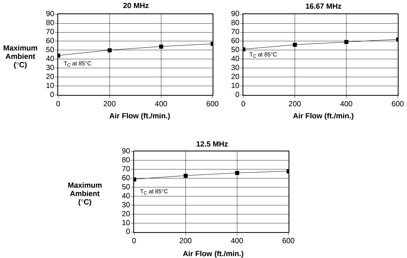
Figure 26. Maximum Allowable Ambient Temperature (Data Sheet Limit, I_{CCOPmax} , V_{CC}=+5.25 V, Average Thermal Impedance)
