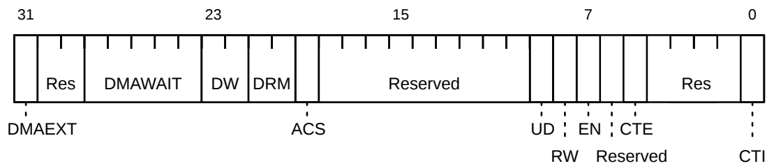
Figure 6. DMA1 Control Register
