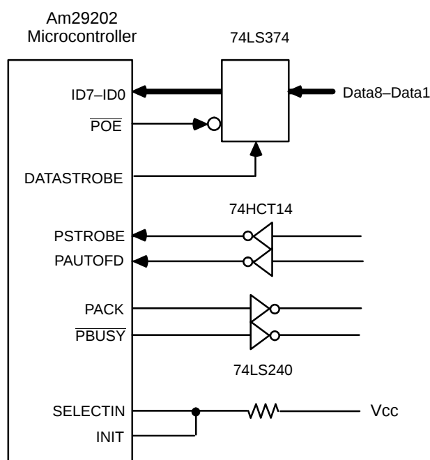
Figure 16. Minimal System Design
