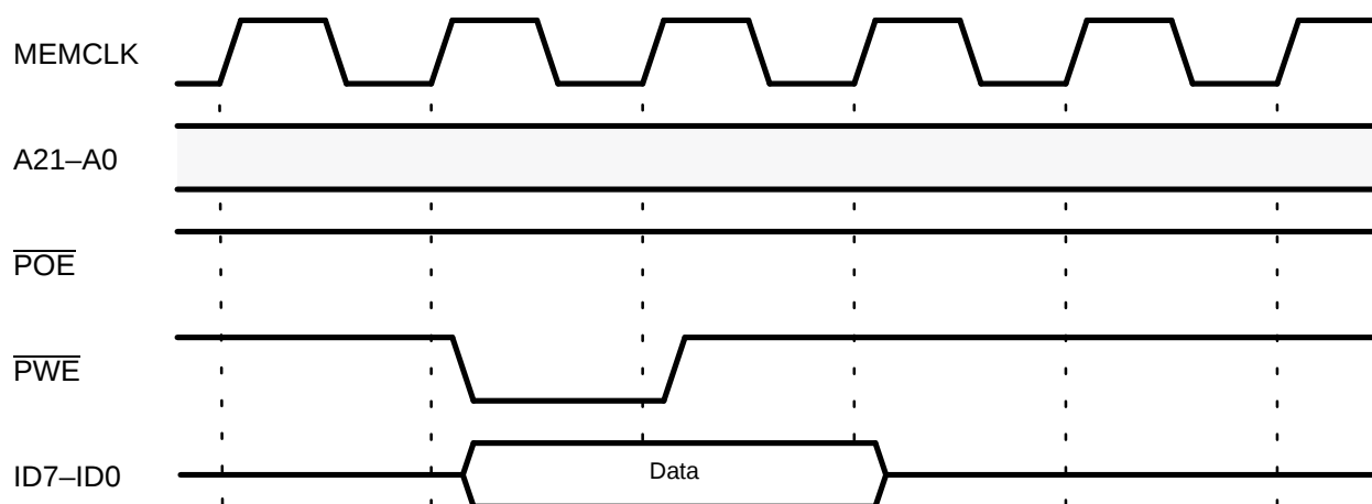
Figure 25. Advanced Parallel Port Buffer Write Cycle for Reverse Transfers
