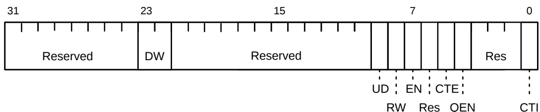
Figure 4. DMA0 Control Register
