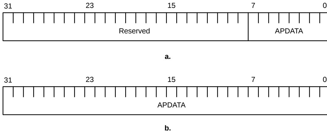
Figure 21. Advanced Parallel Data Register
