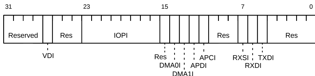
Figure 14. Interrupt Control Register
