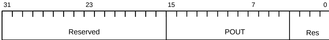
Figure 9. PIO Output Register
