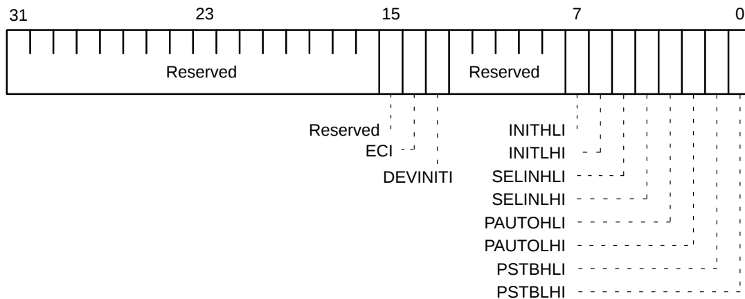
Figure 20. Advanced Parallel Interrupt Status Register
