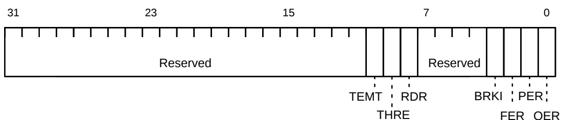
Figure 12. Serial Port Status Register
