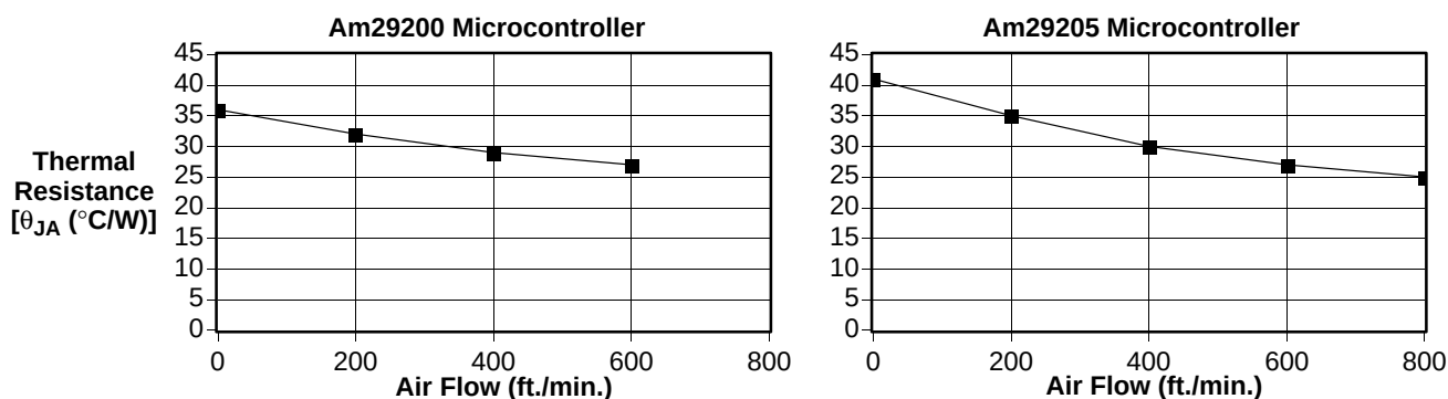
Figure 3. Thermal Impedance
