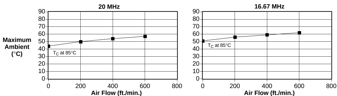
Figure 1. Am29200 Microcontroller—Maximum Allowable Ambient Temperature
