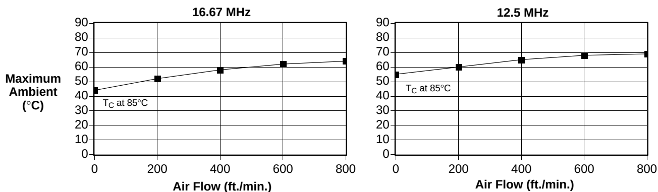
Figure 2. Am29205 Microcontroller—Maximum Allowable Ambient Temperature
