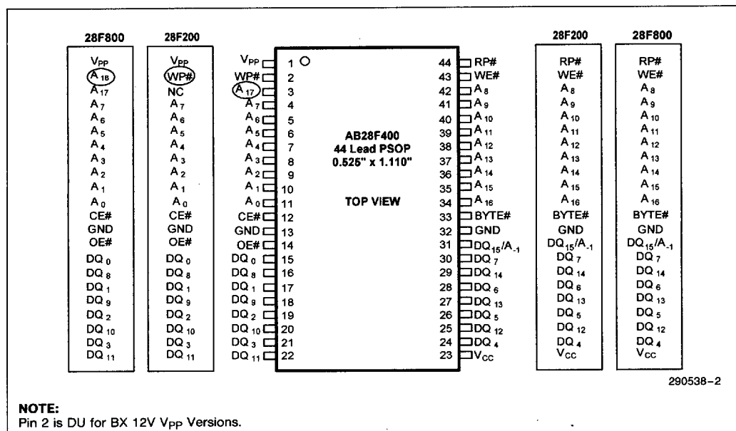
Figure 2. 44-Lead PSOP Lead Configuration for x8/x16 28F400 Is Compatible with 2 and 8 Mbit.
