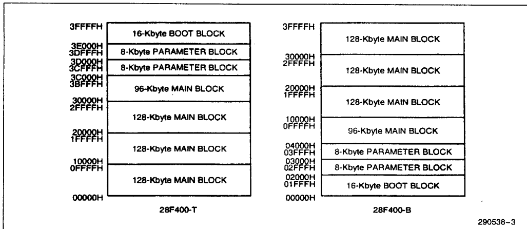
Figure 3. 28F400-T/B Memory Maps
