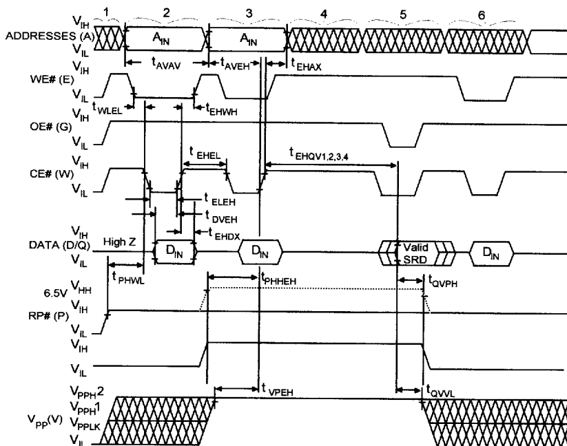
Figure 13. Alternate AC Waveforms for Write and Erase Operations (CE #-Controlled Writes)
