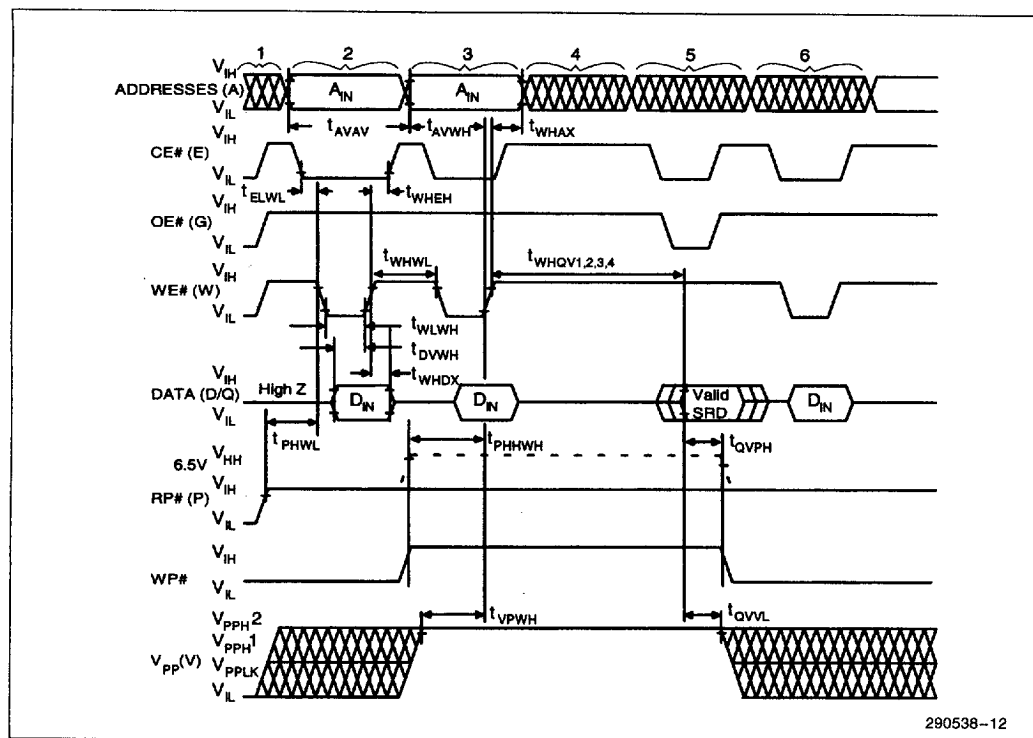
Figure 12. AC Waveforms for Write and Erase Operations (WE#-Controlled Writes)
