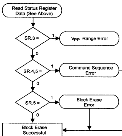
Figure 5. Automated Block Erase Flowchart
