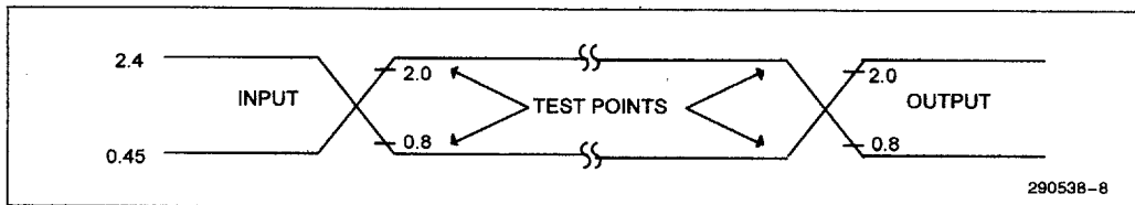
Figure 8. 5V Inputs and Measurement Points
