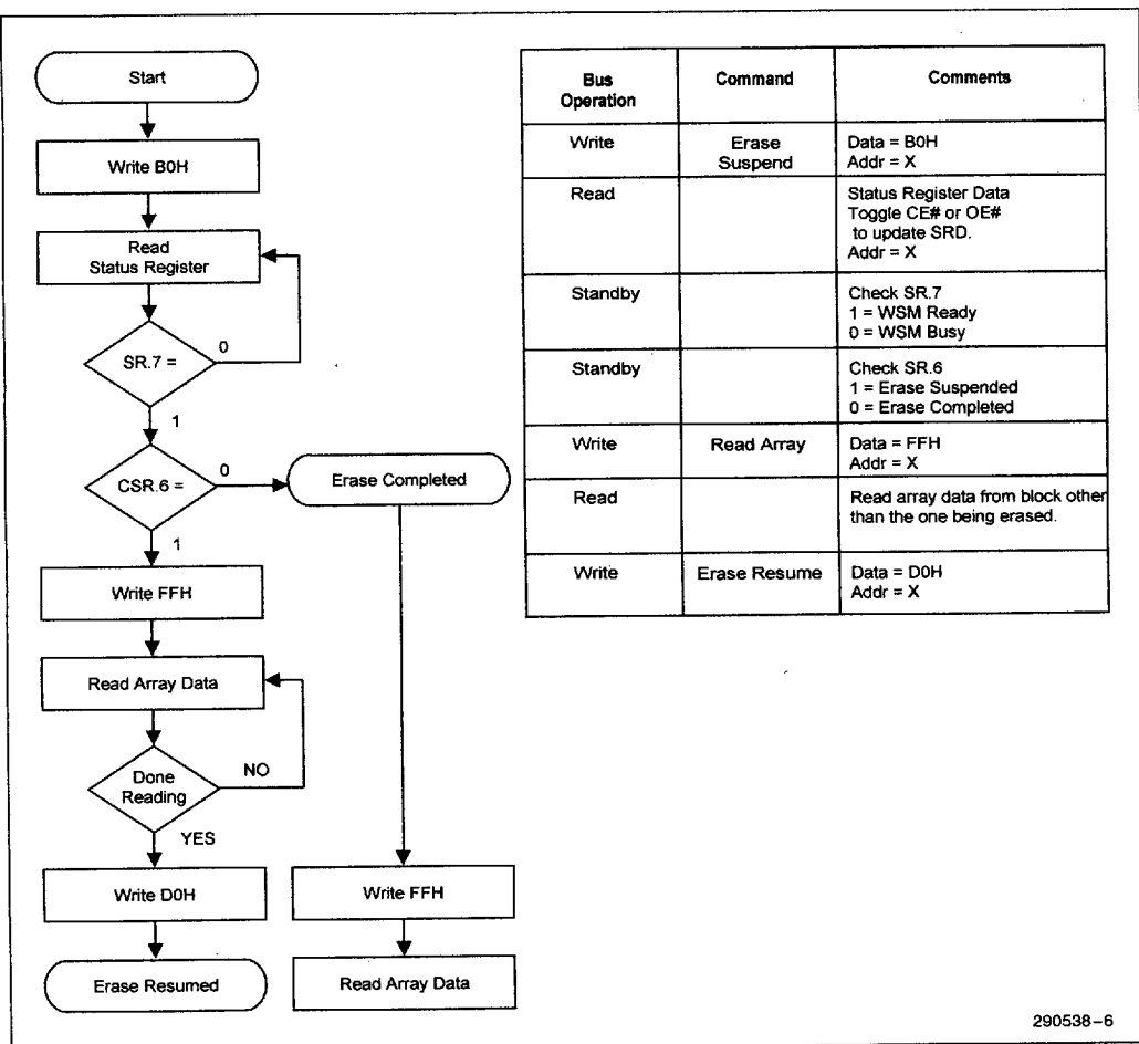
Figure 6. Erase Suspend/Resume Flowchart
