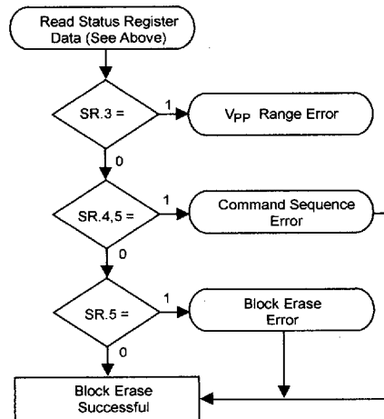
Figure 5. Automated Block Erase Flowchart
