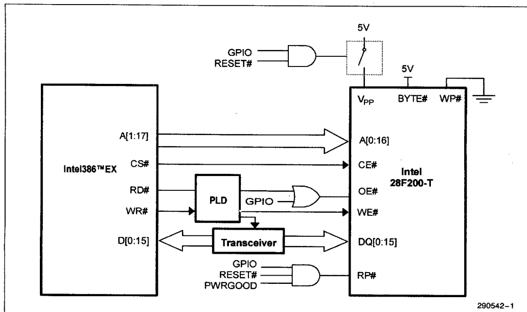
Figure 1. 28F200BX Interface to Intel386™ Microprocessor
