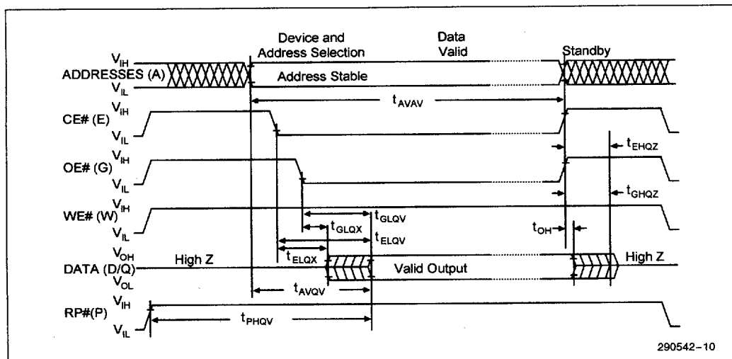
Figure 10. AC Waveforms for Read Operations
