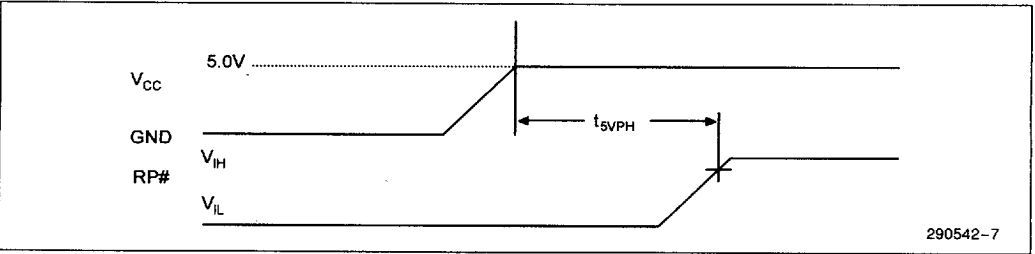
Figure 7. V CC Supply Waveform
