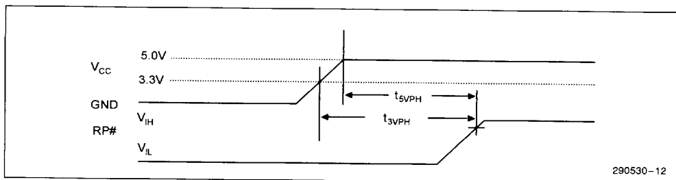
Figure 12. V_{CC} Supply Switching Waveform
