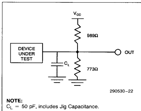
Figure 14. 3.3V Standard Test Configuration
