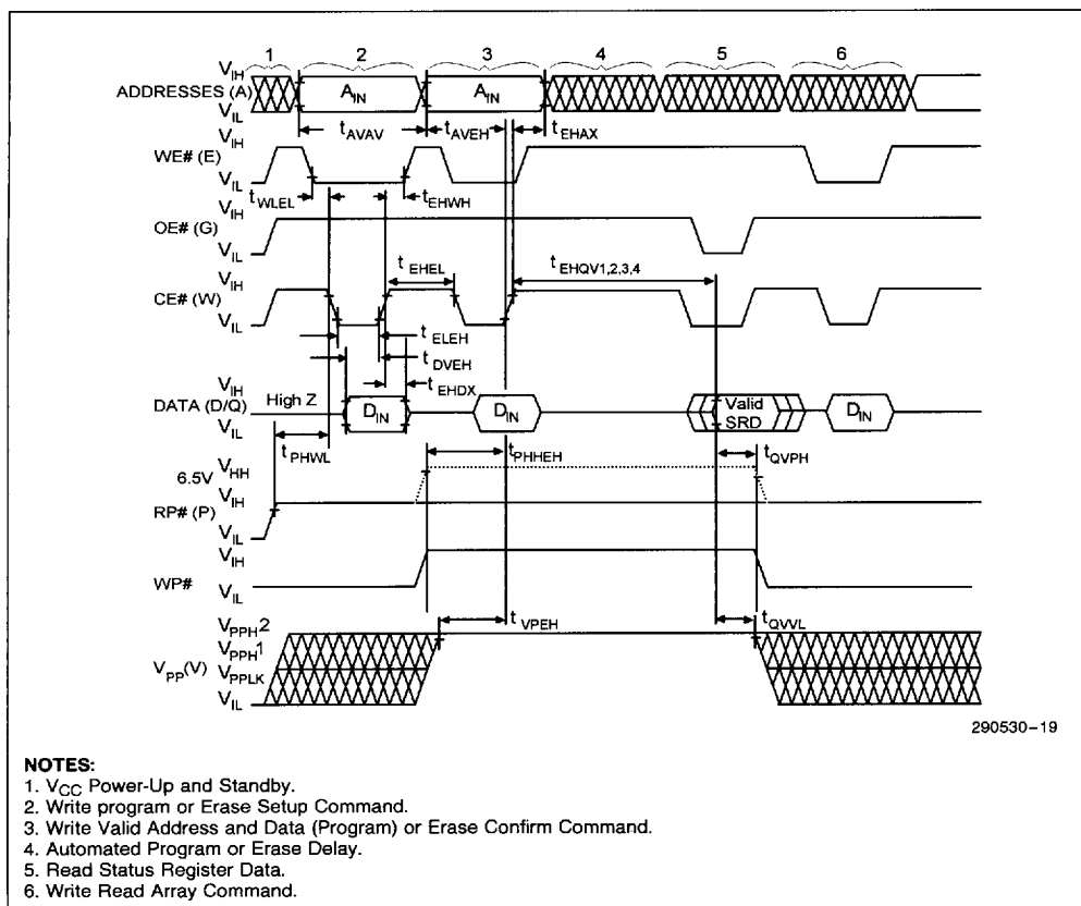
Figure 21. Alternate AC Waveforms for Write and Erase Operations (CE#—Controlled Writes)
