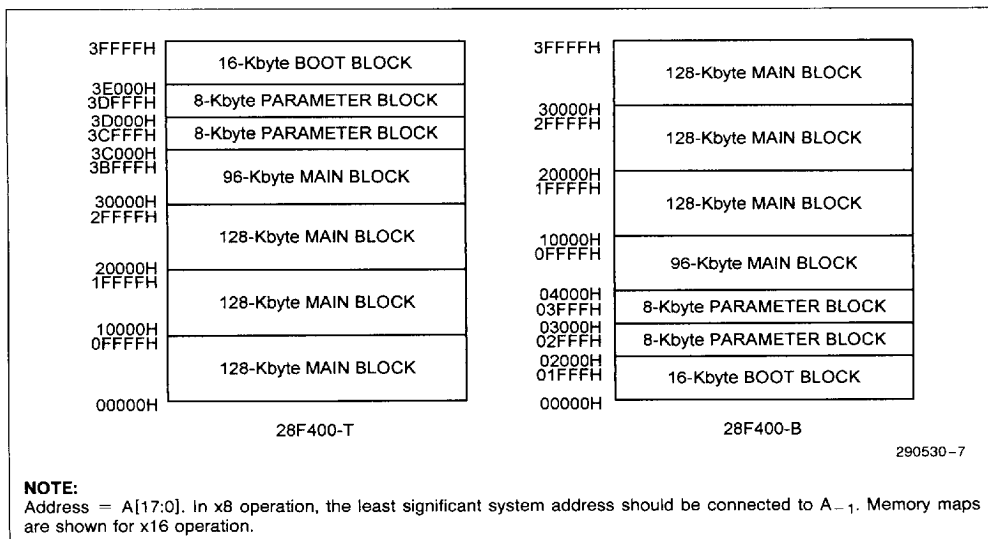
Figure 7. 28F400-T/B Memory Maps
