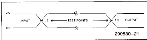
Figure 23. 3.3V Inputs and Measurement Points
