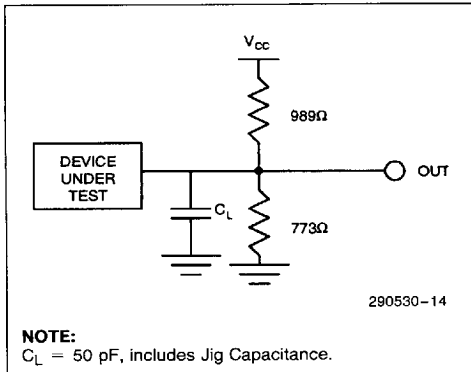
Figure 24. 3.3V Standard Test Configuration
