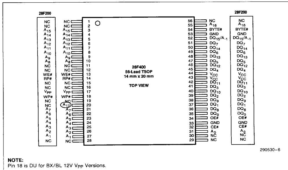
Figure 6. The 56-Lead TSOP Offers Compatibility between 2 and 4 Mbits
