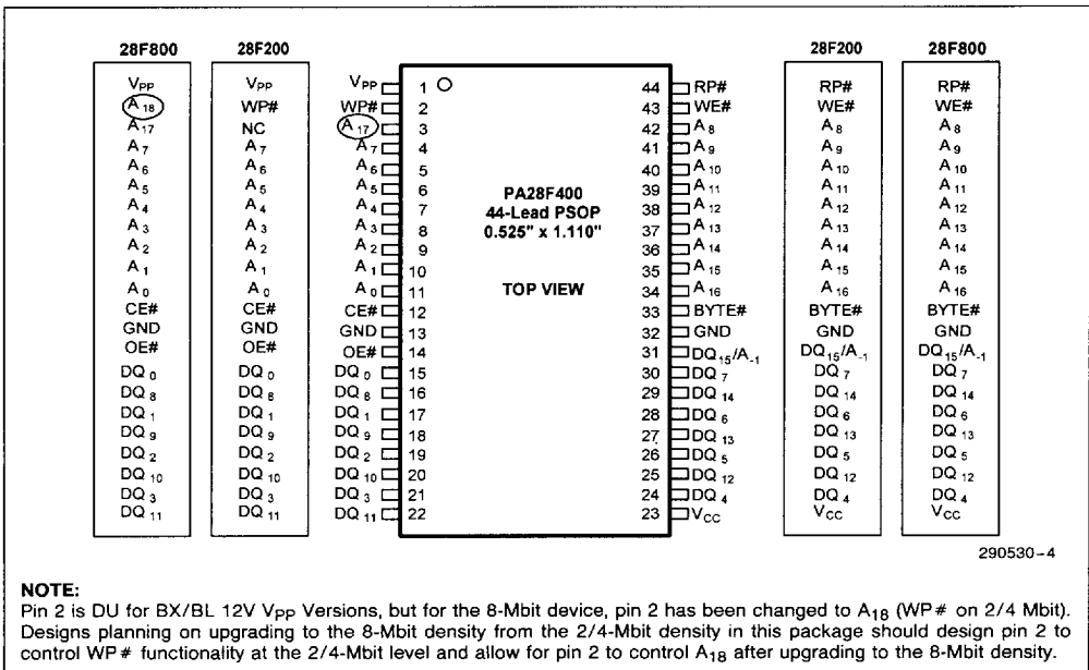
Figure 4. The 44-Lead PSOP Offers a Convenient Upgrade from JEDEC ROM Standards
