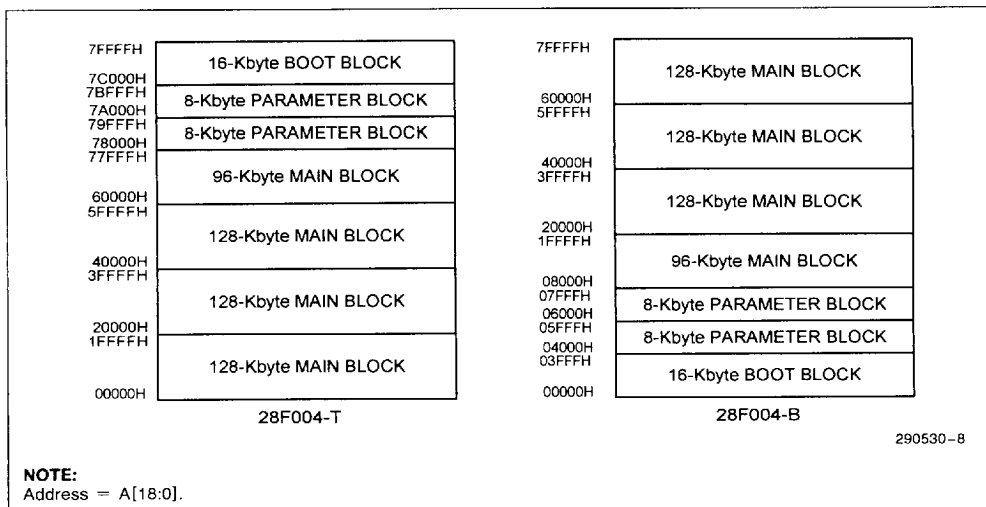
Figure 8. 28F004-T/B Memory Maps
