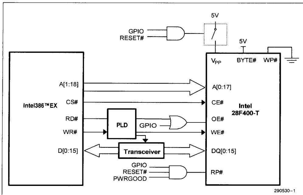
Figure 1. 28F400 Interface to Intel386EX™ Microprocessor
