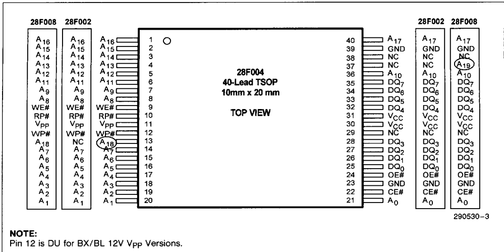
Figure 3. The 40-Lead TSOP Offers the Smallest Form Factor for Space-Constrained Applications
