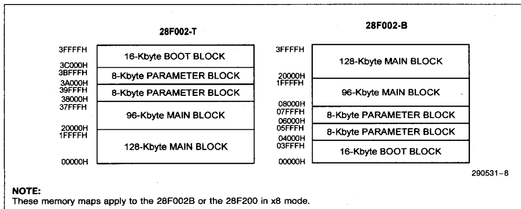
Figure 8. Byte-Wide x8-Mode Memory Maps
