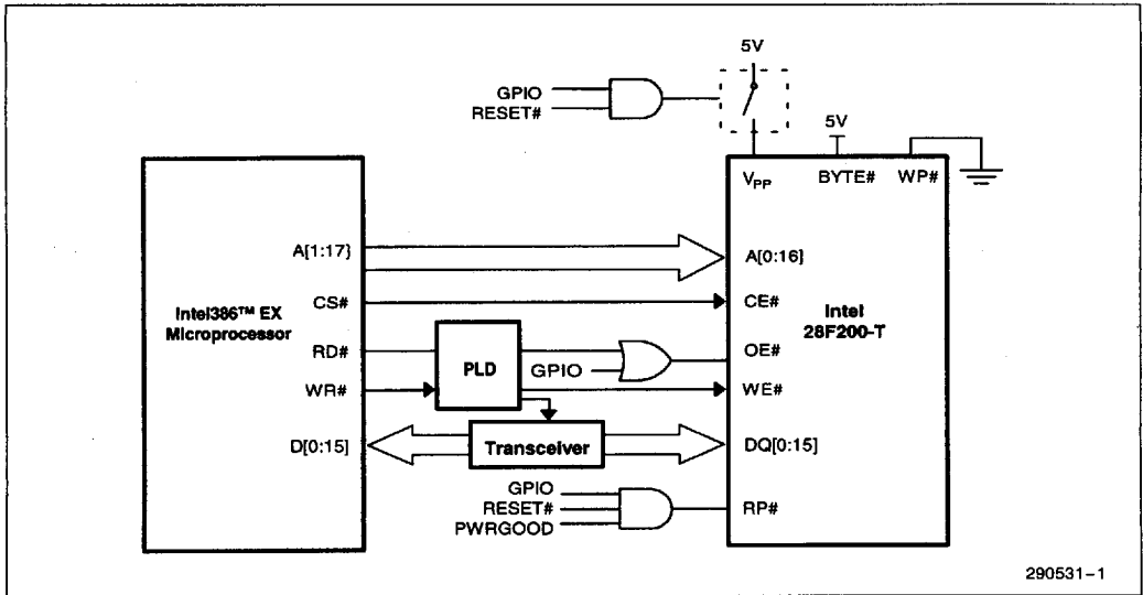
Figure 1. 28F200 Interface to Intel386™ EX Microprocessor
