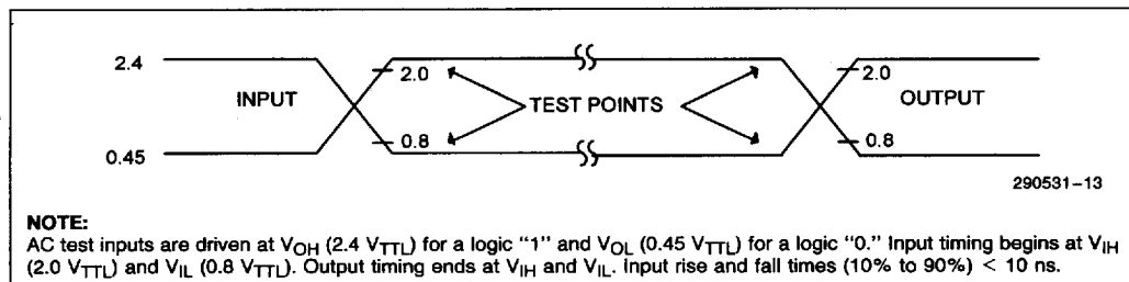
Figure 20. 5V Input Range and Measurement Points
