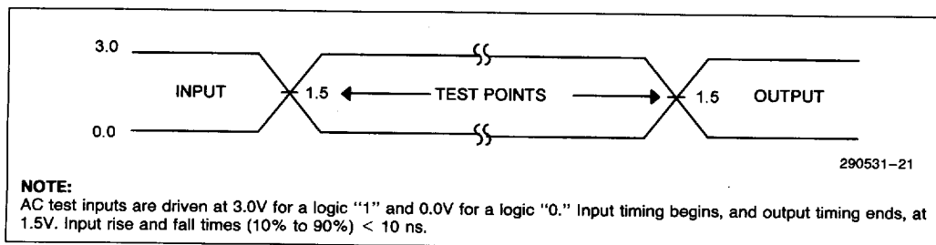
Figure 12. 3.3V Inputs and Measurement Points
