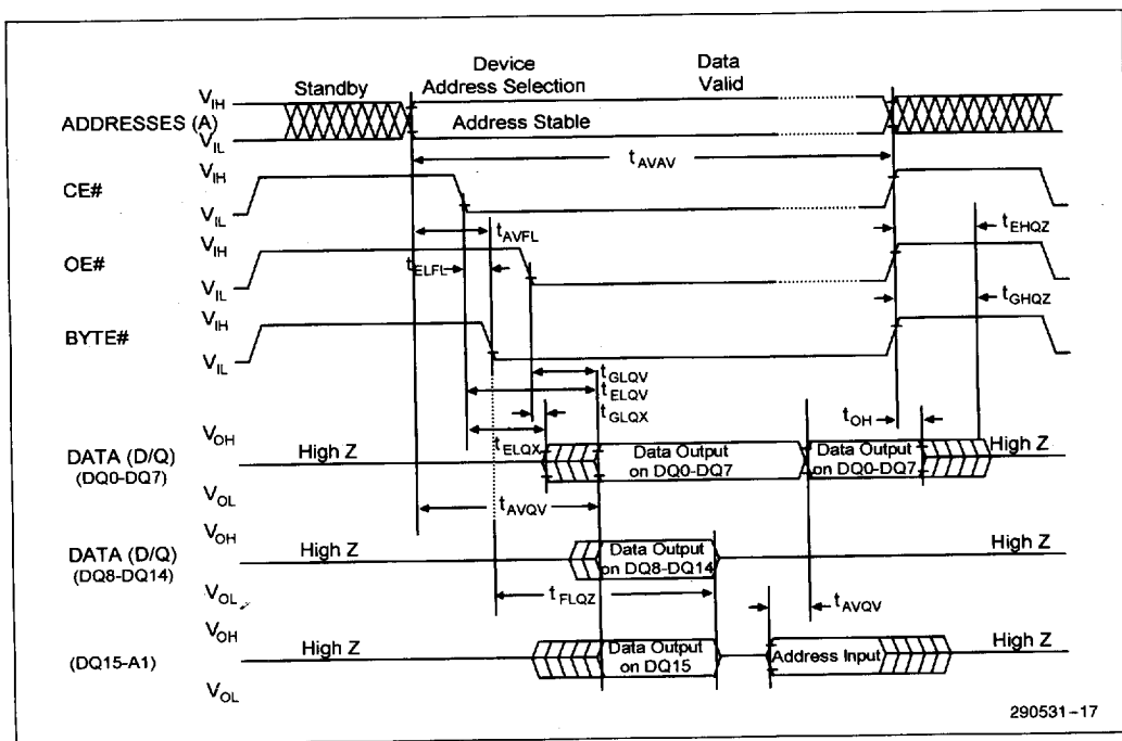
Figure 16. BYTE # Timing Diagram for Read Operations
