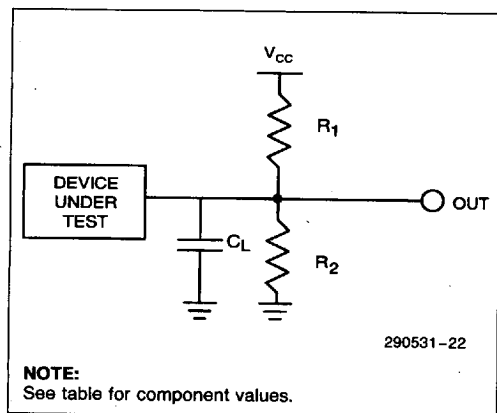
Figure 14. Test Configuration
