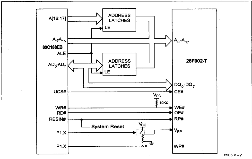
Figure 2. 28F002B Interface to Intel80C188EB 8-Bit Embedded Microprocessor
