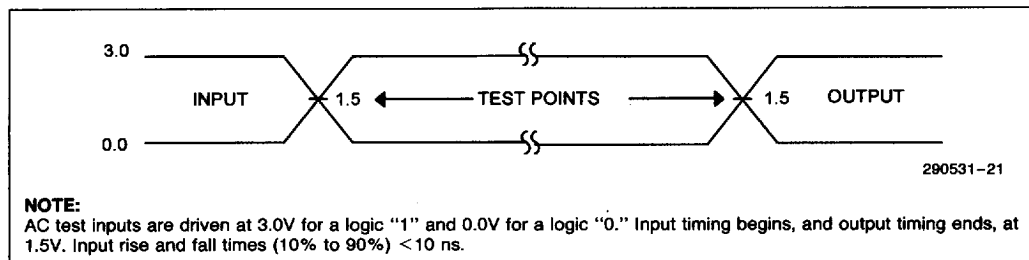
Figure 19. 3.3V Input Range and Measurement Points
