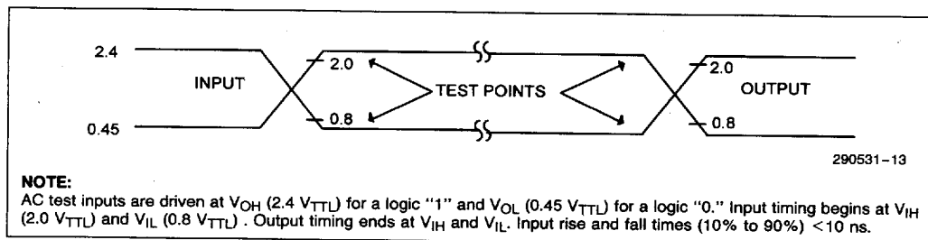
Figure 13. 5V Inputs and Measurement Points
