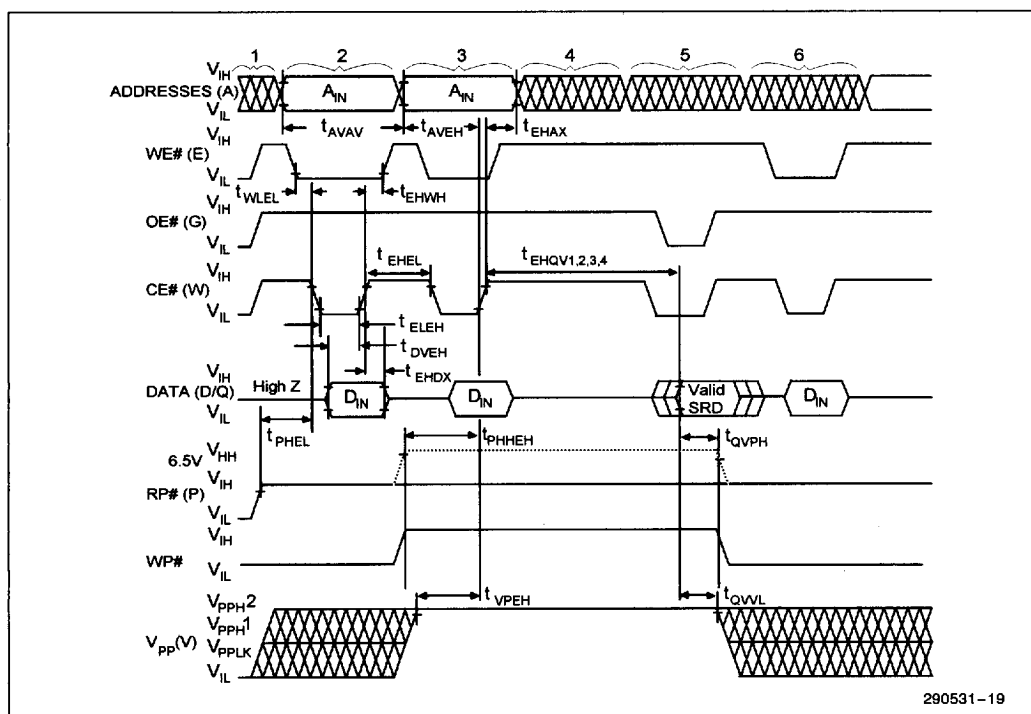
Figure 18. Alternate AC Waveforms for Write and Erase Operations (CE# - Controlled Writes)
