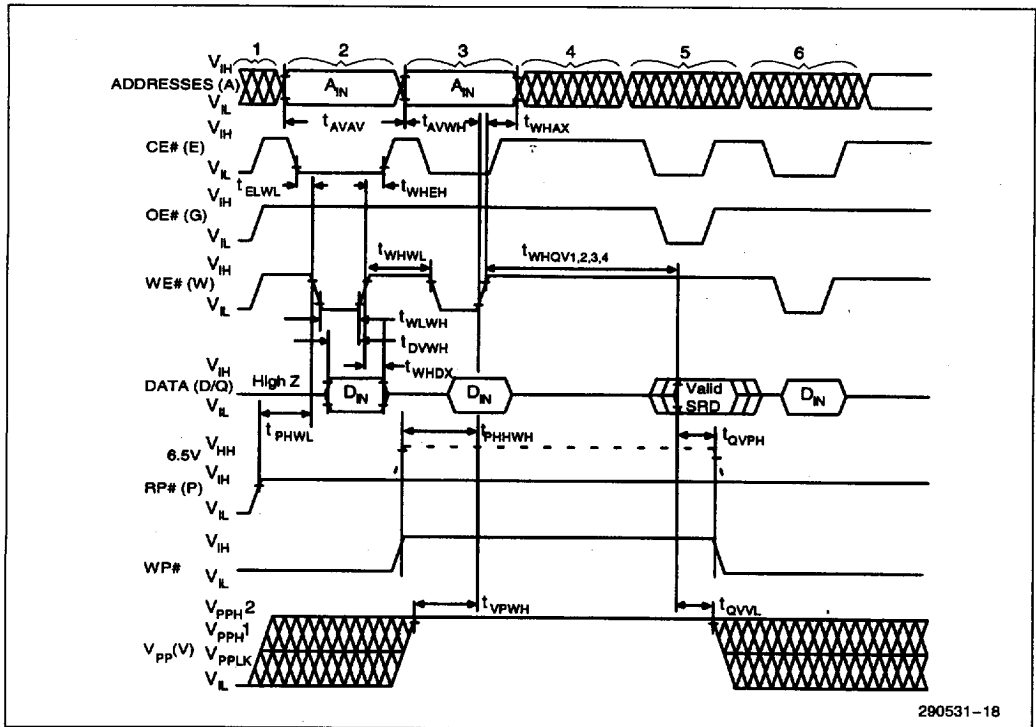
Figure 17. AC Waveforms for Write and Erase Operations (WE#-Controlled Writes)
