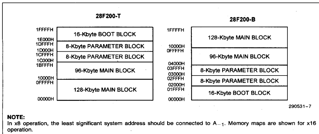
Figure 7. Word-Wide x16-Mode Memory Maps
