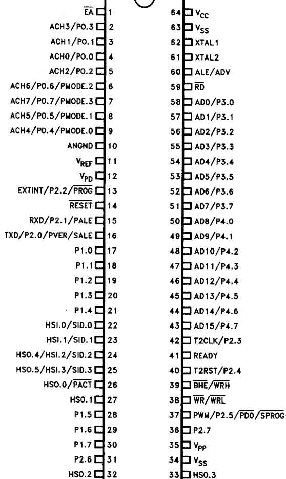
Figure 6. Shrink-DIP Package
