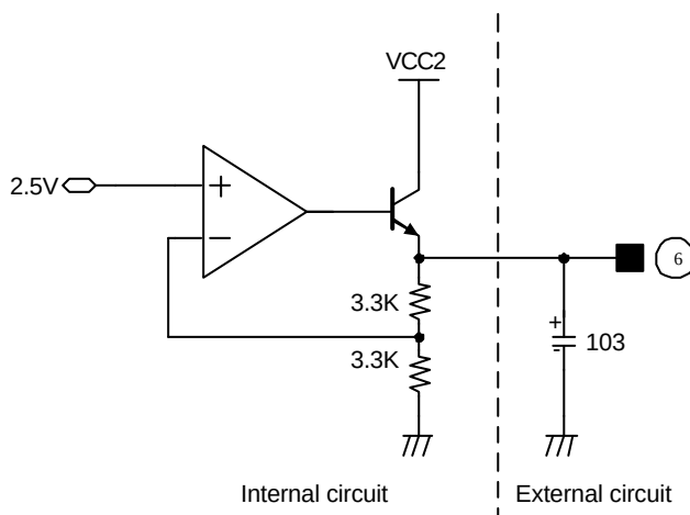
Fig7. Regulator
