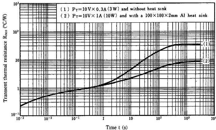
R_{th(t)} - t
