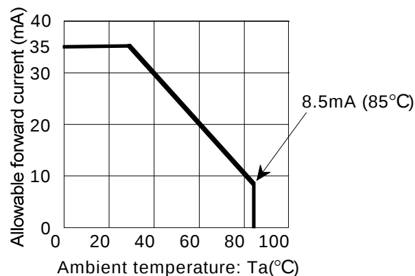
Fig.1 Ambient Temperature vs. Allowable Forward Current
