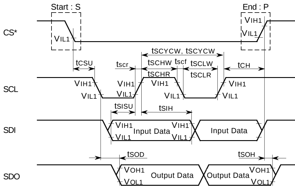
Clock Synchronized Serial Interface (SPI) Timing
