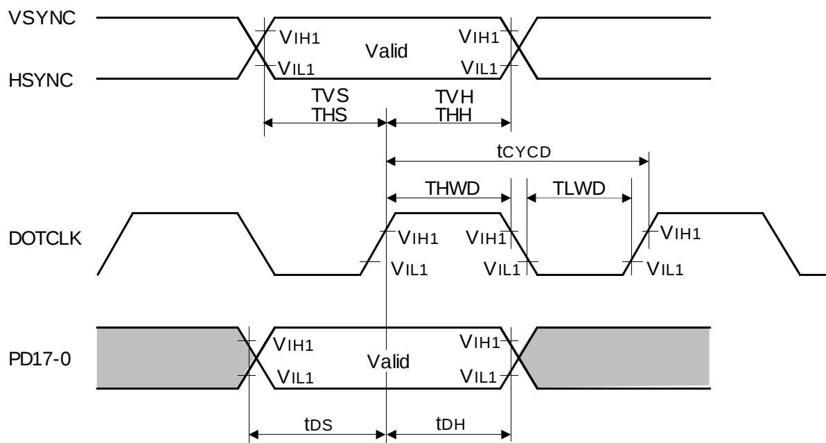
RGB Interface Timing
