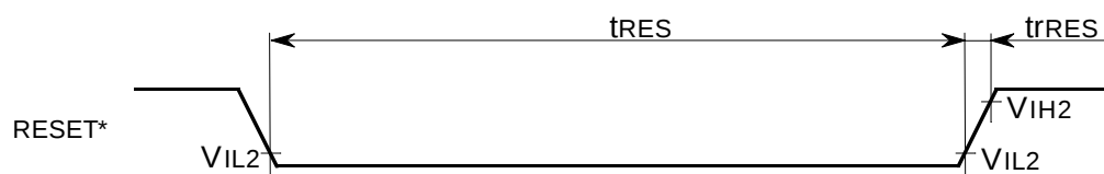
Reset Timing
