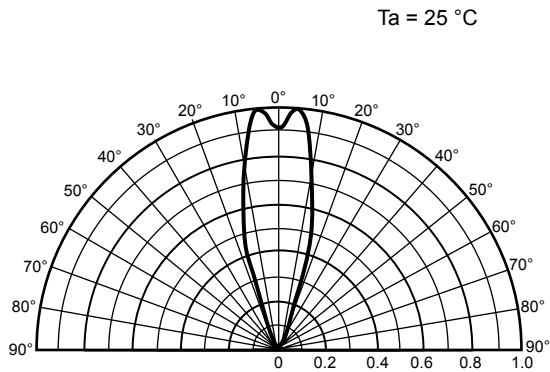
Radiation Pattern
