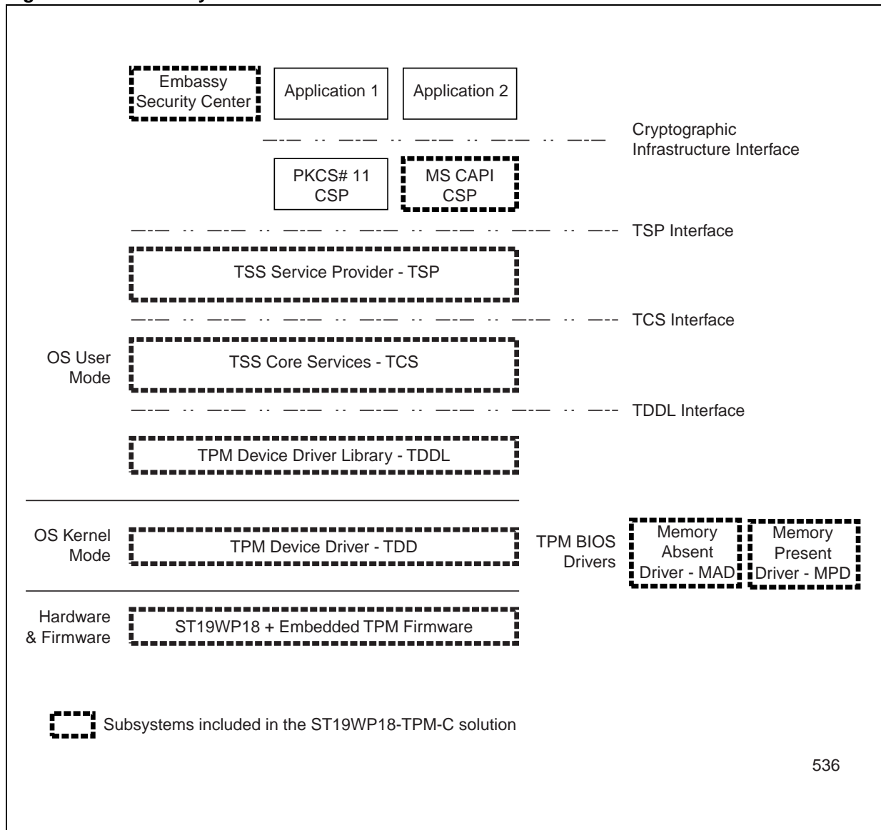
Figure 3. Software Layers
