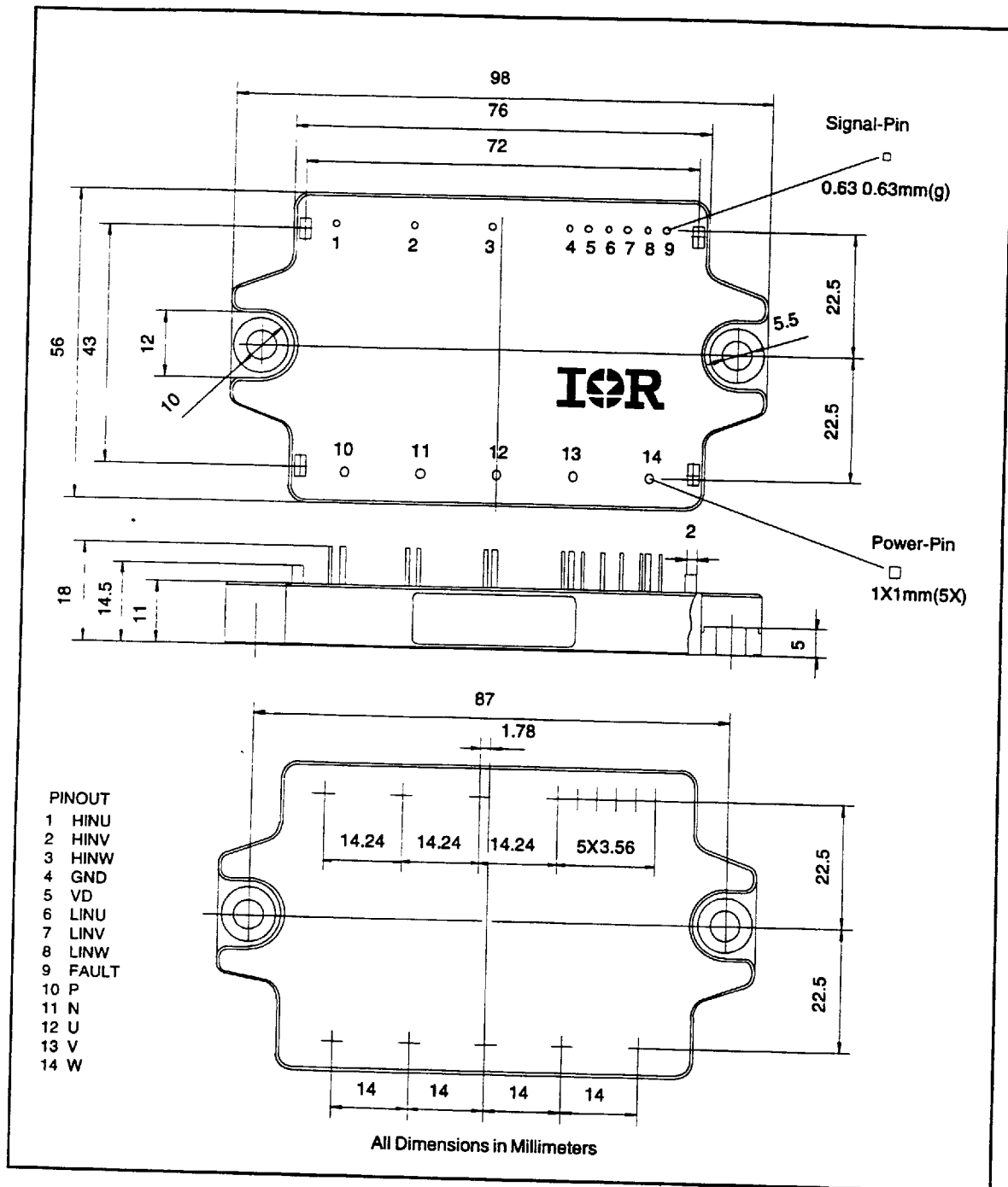
Fig. 7 - Package Outline
