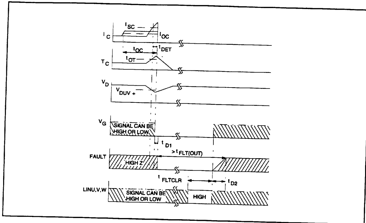
Fig. 10 - Timing Diagram
