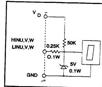
Figure 8 : Input Stage
