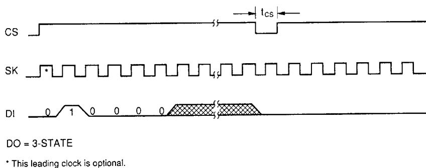
FIGURE 7. WRITE DISABLE (WDS) CYCLE TIMING
