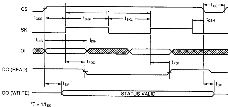
FIGURE 2. SYNCHRONOUS DATA TIMING
