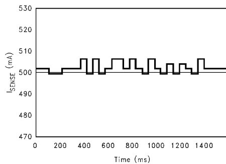
FIGURE 9. Typical Response of LM3812PM-1.0/LM3813PM-1.0 (Precision Mode Operation)
