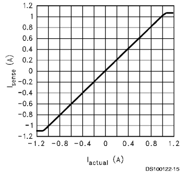
Measured Current vs Actual Current (LM3812-1.0 and LM3813-1.0)
