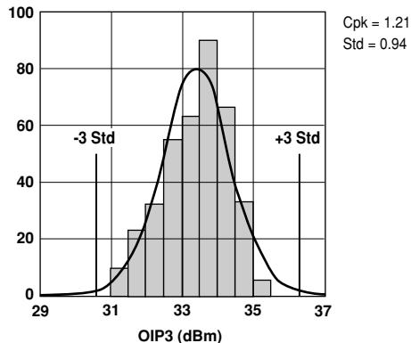
Figure 3. OIP3 @ 2 GHz, 4 V, 80 mA. LSL=30.0, Nominal=33.3, USL=37.0
