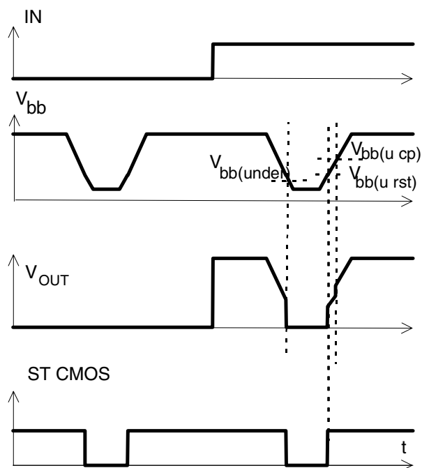
Figure 6a: Undervoltage:
