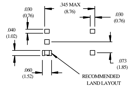
PWB FOOTPRINT
