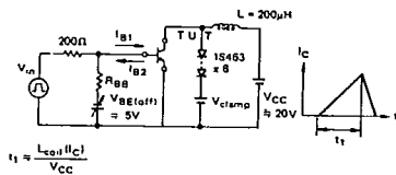
Test Circuit for V_{CEX(sus)} and Reverse Bias Safe Operating Area
