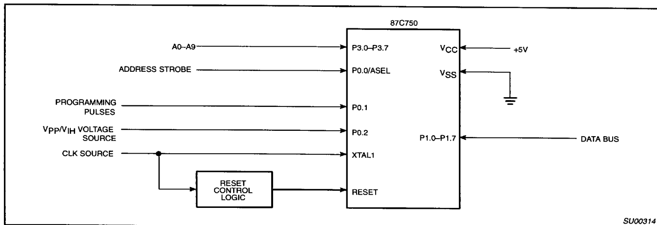
Figure 4. Programming Configuration
