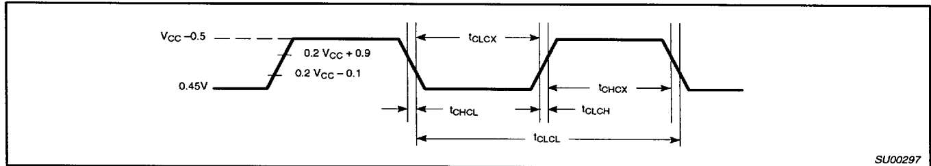
Figure 2. External Clock Drive
