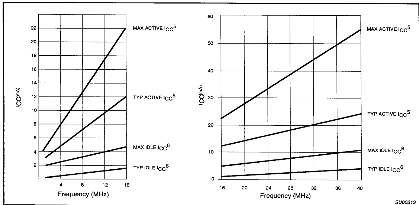
Figure 3. I_{CC} vs. Frequency
