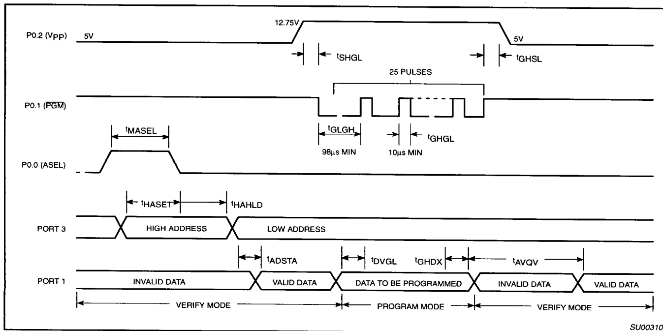
Figure 6. Program/Verify Cycle
