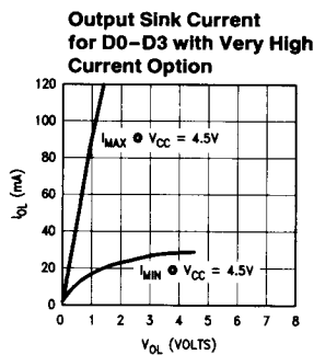
FIGURE 8b. COP310L/COP311L Input/Output Characteristics
