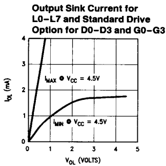
FIGURE 8b. COP310L/COP311L Input/Output Characteristics
