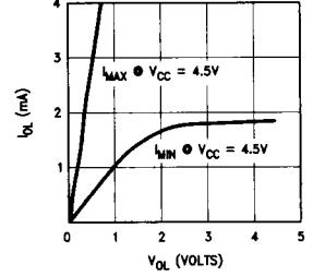
Output Sink Current for D0-D3 (for High Current Option)
