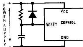
FIGURE 5. Power-Up Clear Circuit
