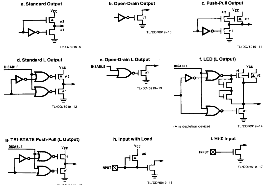
FIGURE 7. Input and Output Configurations
