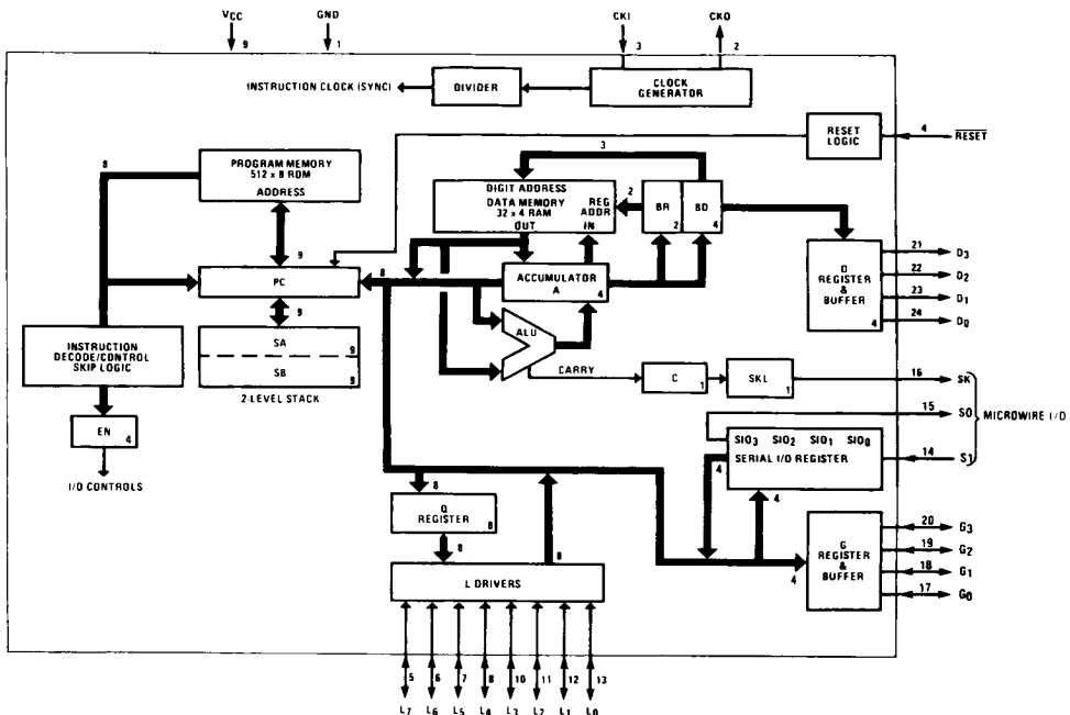
FIGURE 1. COP410L
