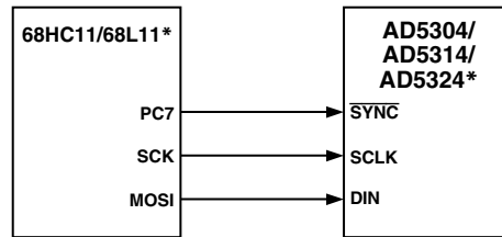
Figure 11. AD5304/AD5314/AD5324 to 68HC11/68L11 Interface
