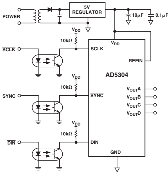
Figure 16. AD5304 in an Opto-Isolated Interface
