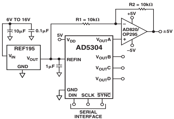
Figure 15. Bipolar Operation with the AD5304
