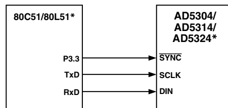
Figure 12. AD5304/AD5314/AD5324 to 80C51/80L51 Interface
