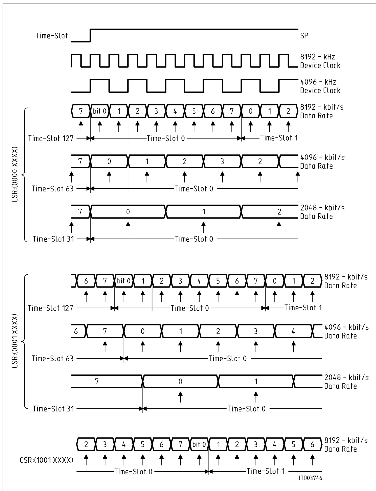
Figure 9 Latching Instant for Input Data
