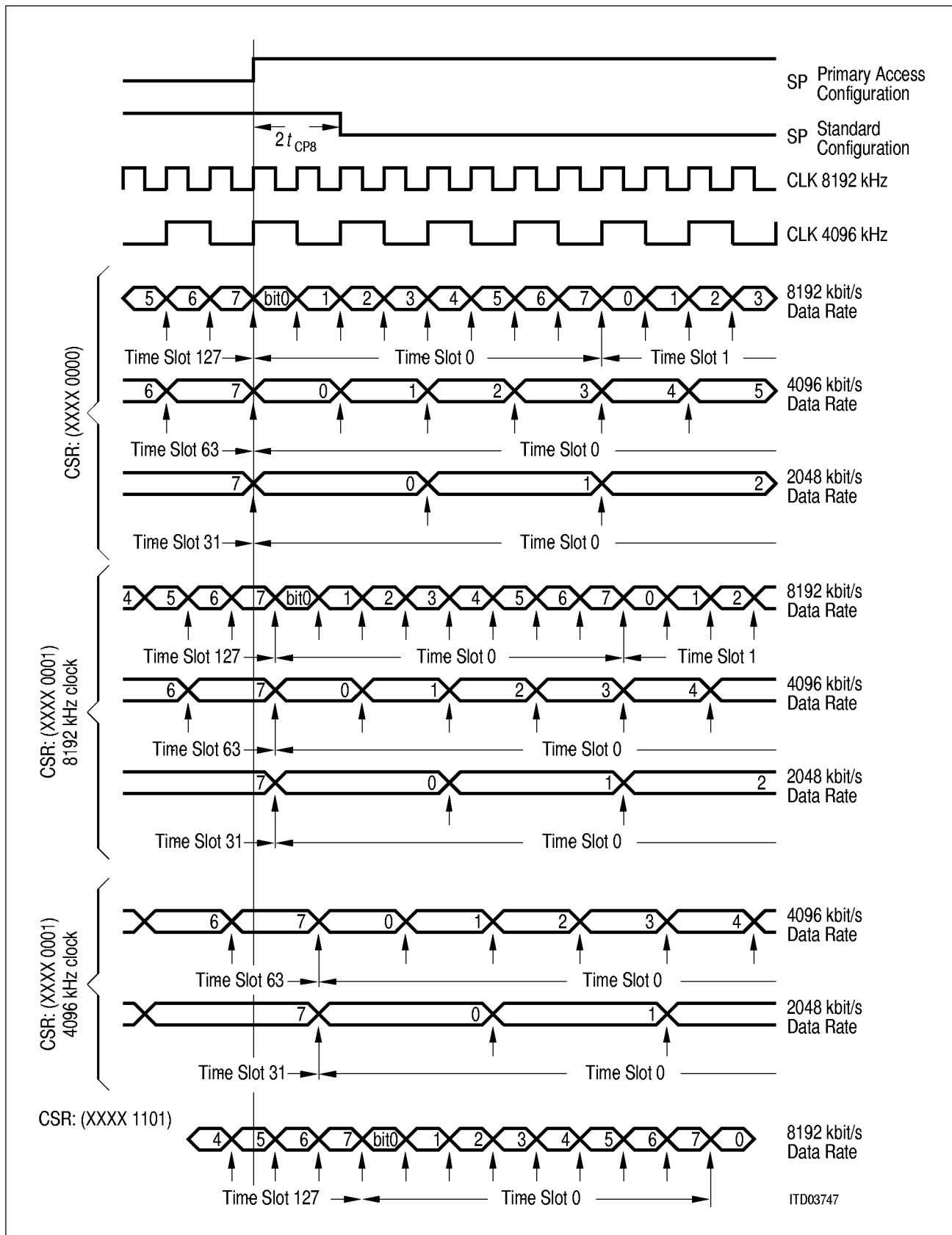
Figure 11 Clocking Off Instant of Output Data
