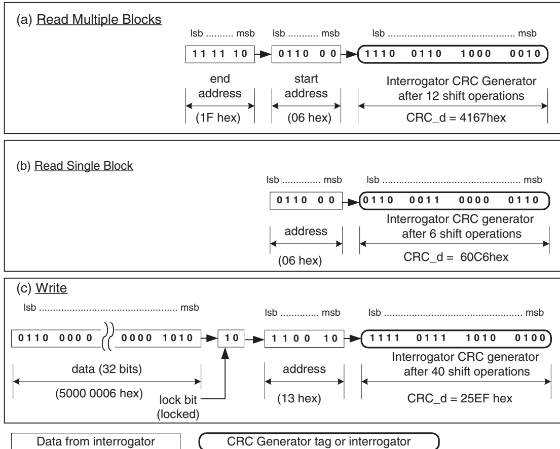
Figure 4-2. Examples of Downlink CRC Generation
