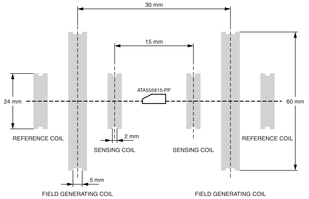
Figure 9-3. Testing Geometry
