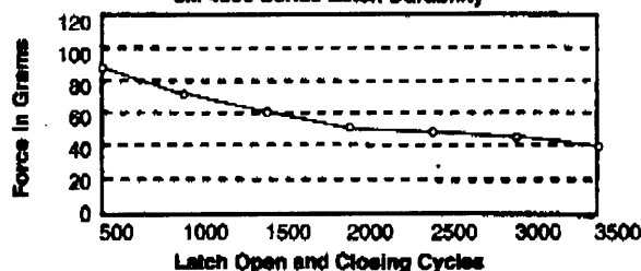
3M 4800 Series Latch Durability
