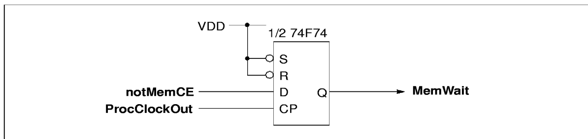
Figure 5.10 Single wait state generator
