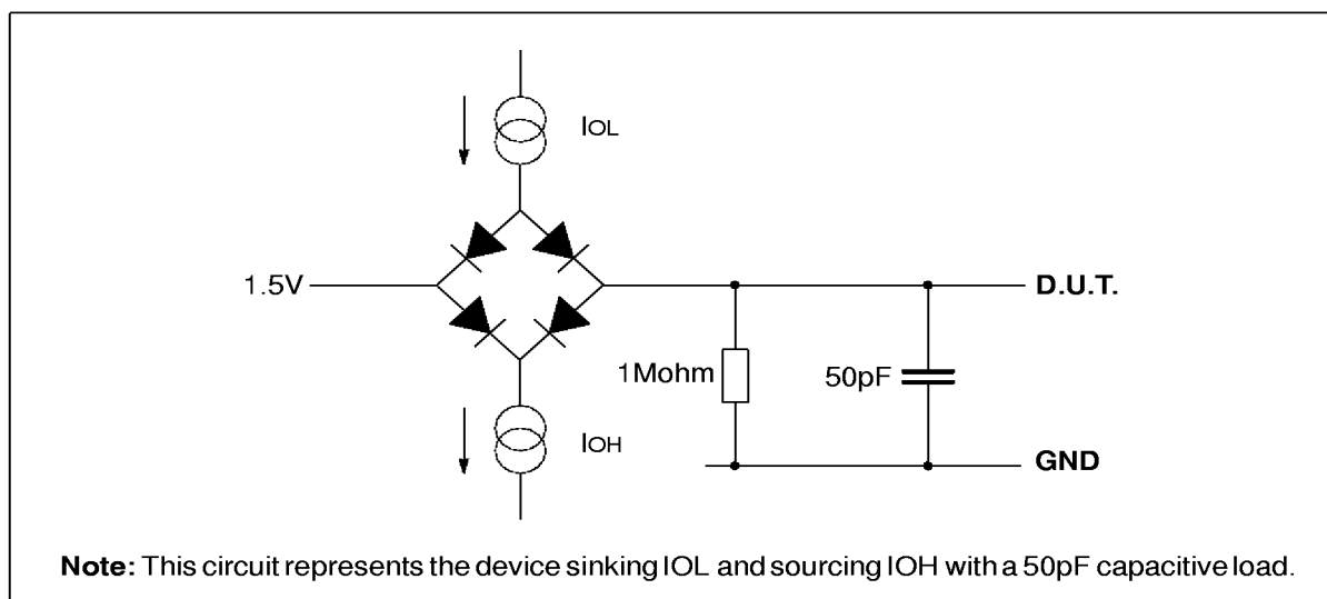
Figure 8.1 Load circuit for AC measurements
