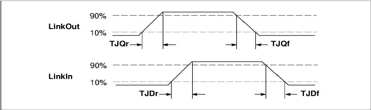
Figure 7.2 IMS T225E link timing
