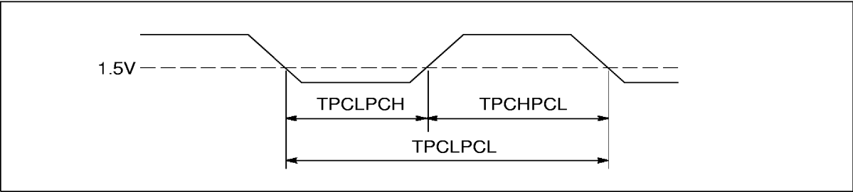
Figure 5.3 IMS T225E ProcClockOut timing
