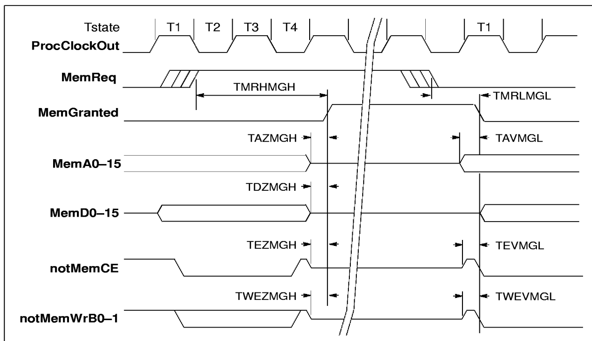
Figure 5.14 IMS T225E memory request timing
