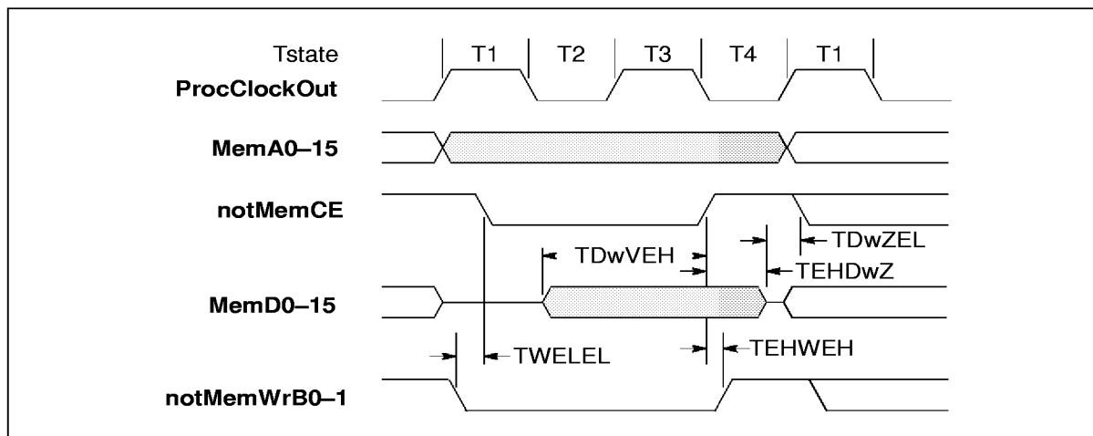
Figure 5.5 IMS T225E external write cycle
