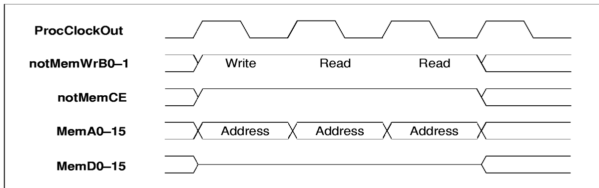
Figure 5.1 IMS T225E bus activity for 3 internal memory cycles
