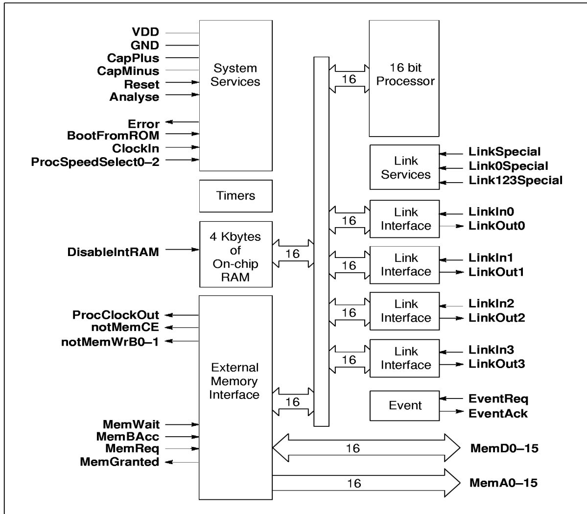
Figure 1.1 IMS T225E block diagram
