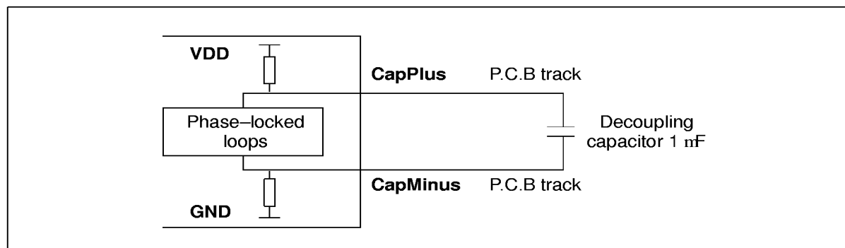
Figure 3.1 Recommended PLL decoupling
