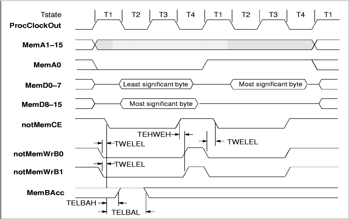
Figure 5.7 IMS T225E word write to byte-wide memory
