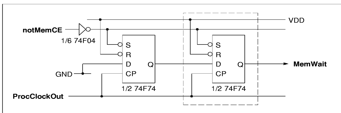
Figure 5.11 Extendable wait state generator
