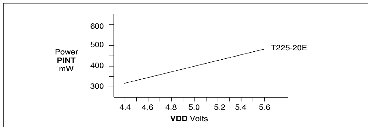
Figure 8.5 IMS T225E internal power dissipation vs VDD
