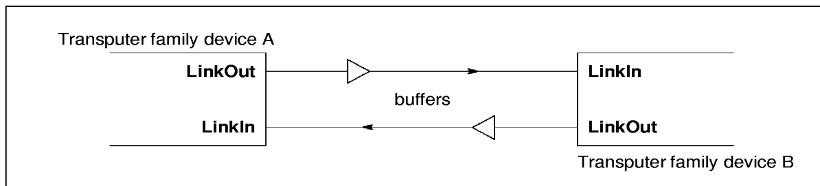
Figure 7.6 IMS T225E links connected by buffers
