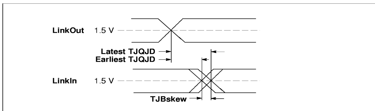
Figure 7.3 IMS T225E buffered link timing
