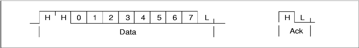
Figure 7.1 IMS T225E link data and acknowledge packets
