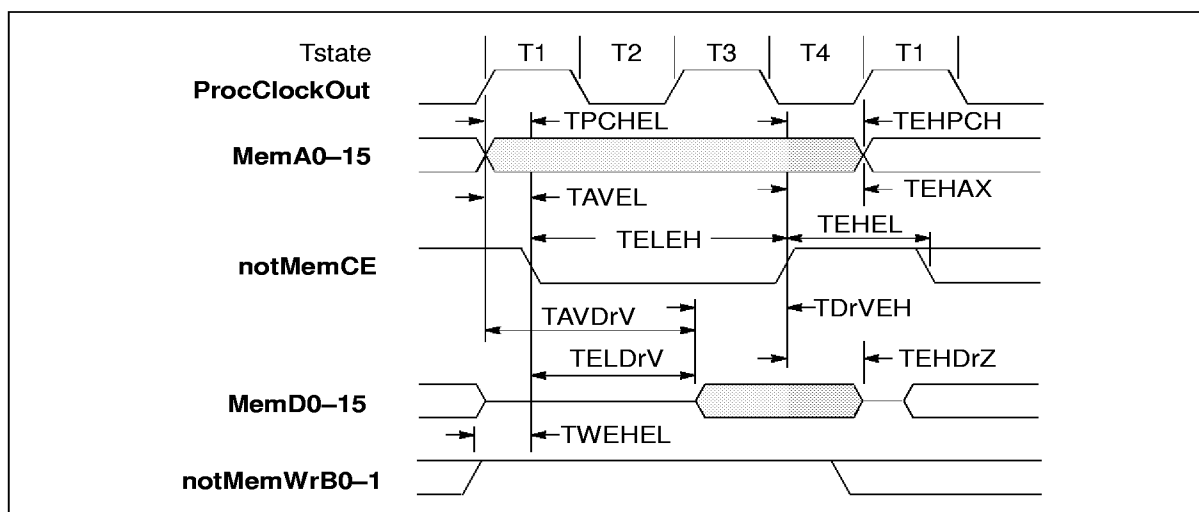
Figure 5.4 IMS T225E external read cycle
