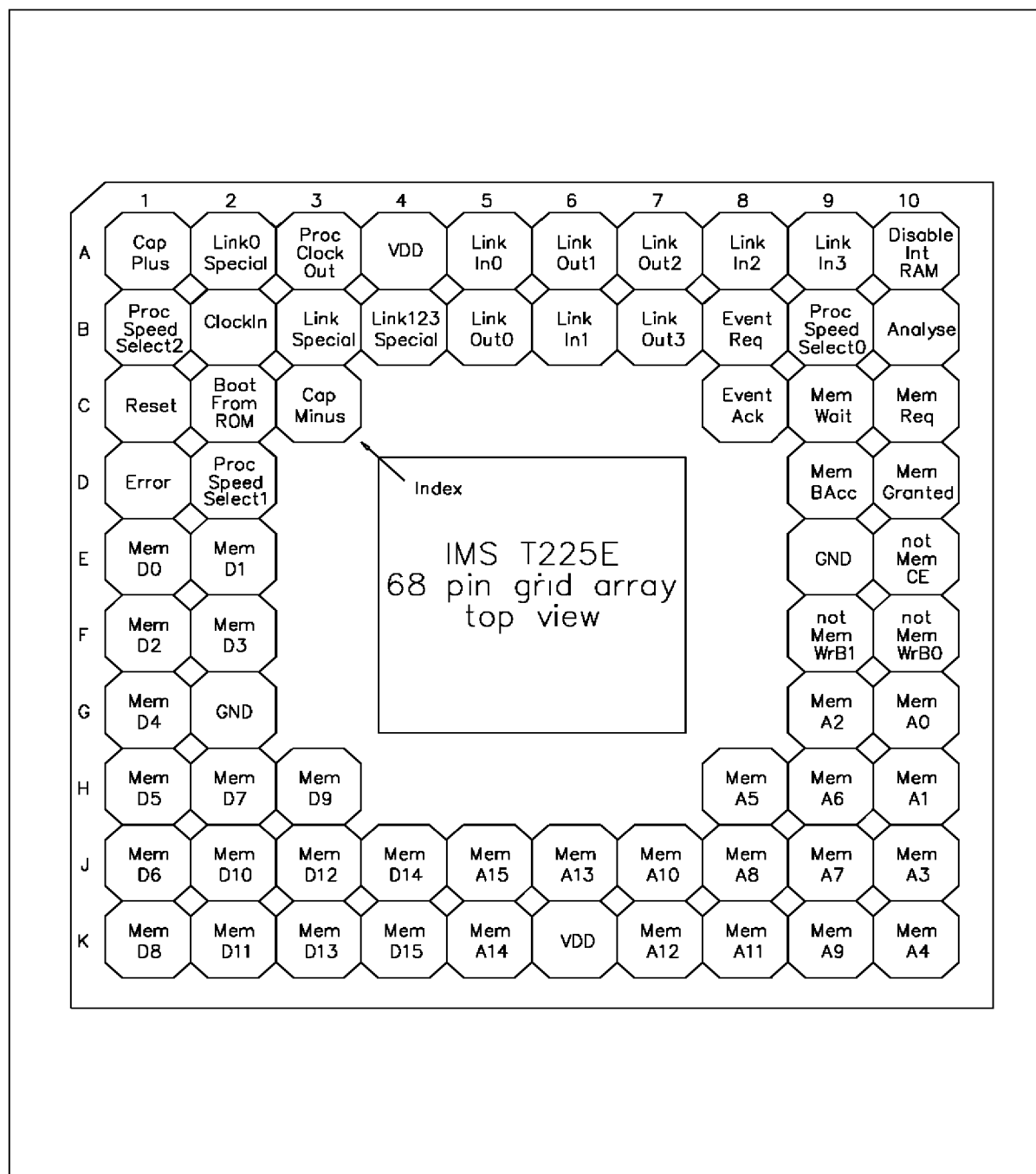
Figure 9.1 IMS T225E 68 pin grid array package pinout
