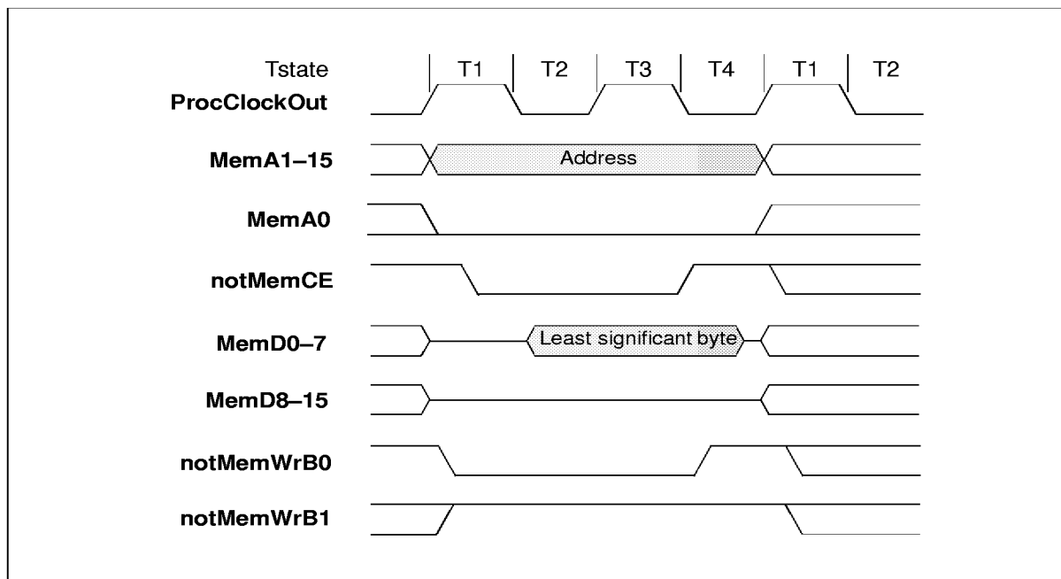
Figure 5.6 IMS T225E least significant byte write in word access mode
