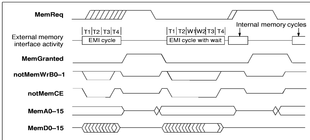
Figure 5.13 IMS T225E operation of MemReq and MemGranted with external and internal memory cycles
