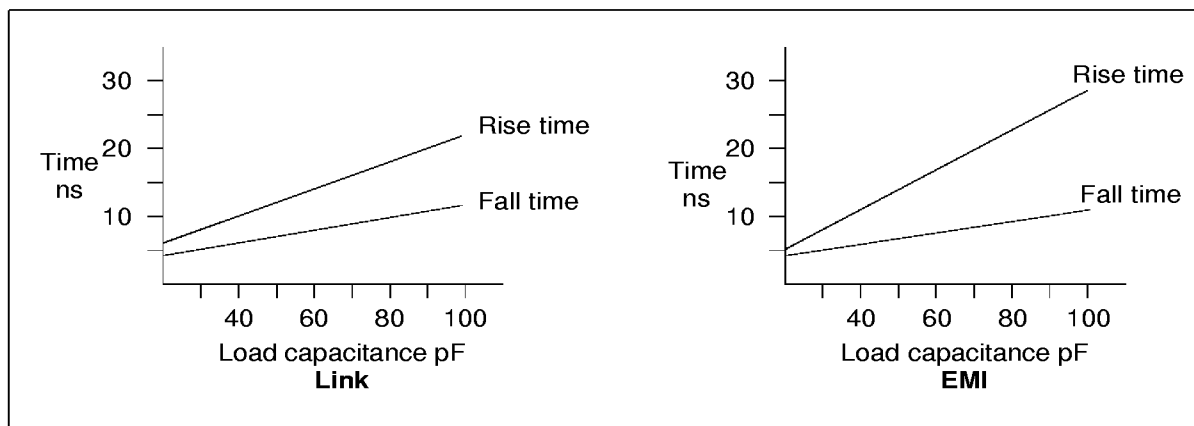
Figure 8.4 Typical rise/fall times
