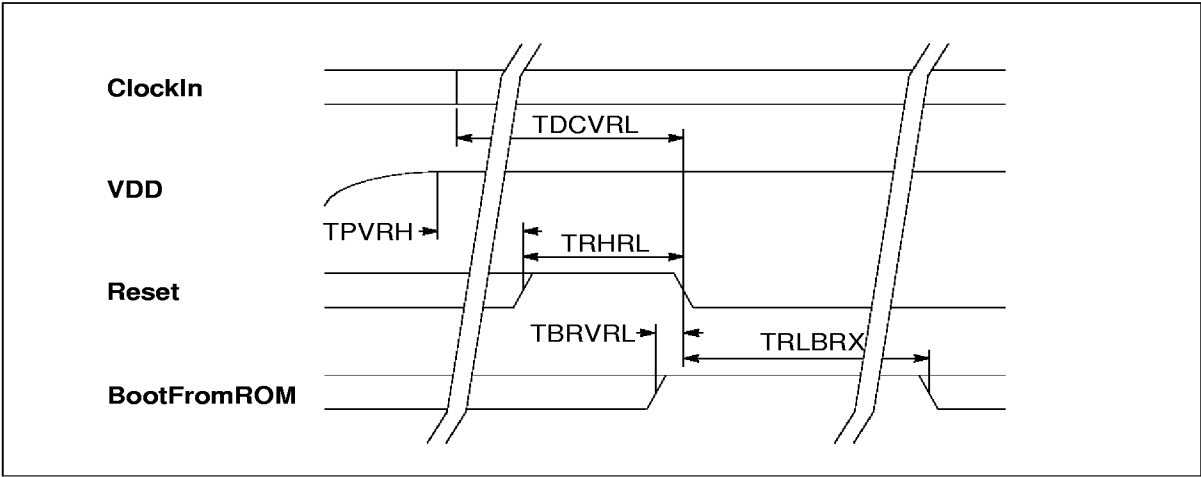
Figure 3.3 Transputer Reset timing with Analyse low
