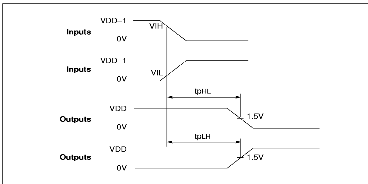
Figure 8.2 AC measurements timing waveforms
