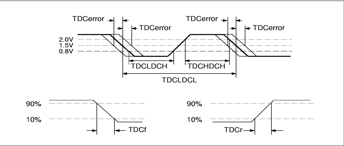
Figure 3.2 ClockIn timing
