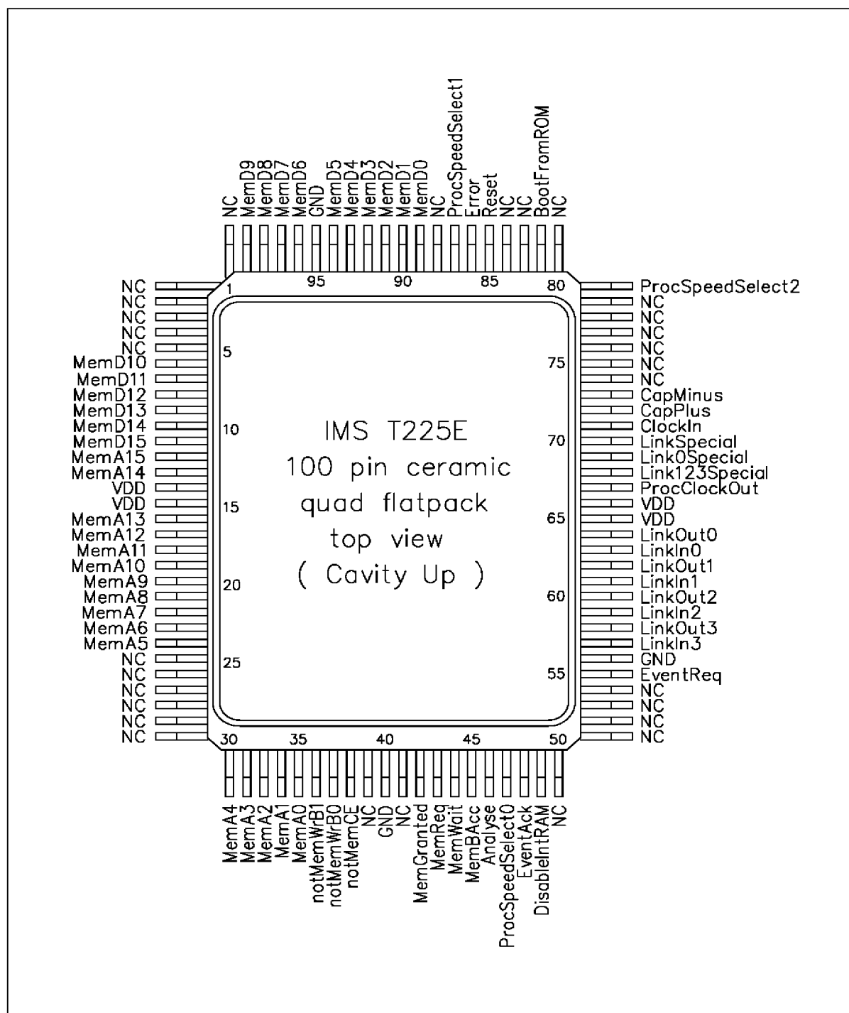
Figure 9.3 IMS T225E 100 pin cavity-up ceramic quad flat pack package pinout
