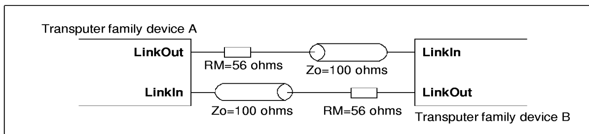
Figure 7.5 IMS T225E links connected by transmission line
