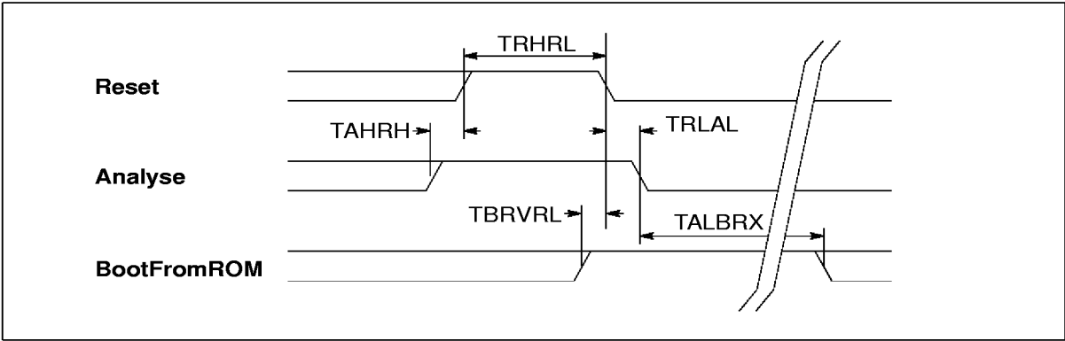
Figure 3.4 Transputer Reset , Analyse and BootFromROM timing
