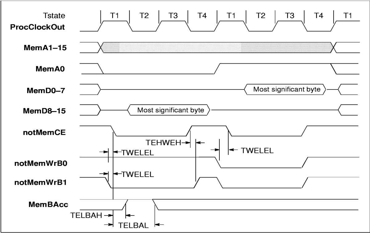
Figure 5.8 IMS T225E most significant byte write to byte-wide memory
