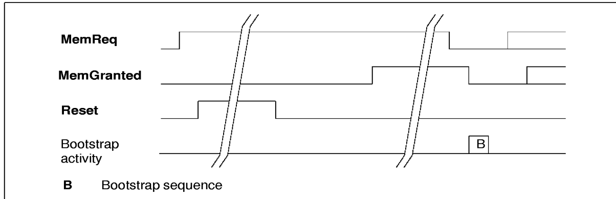
Figure 5.12 IMS T225E DMA sequence at reset
