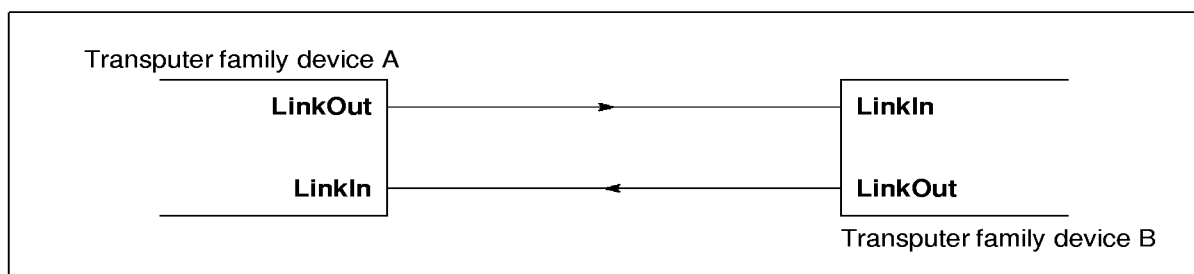
Figure 7.4 IMS T225E links directly connected
