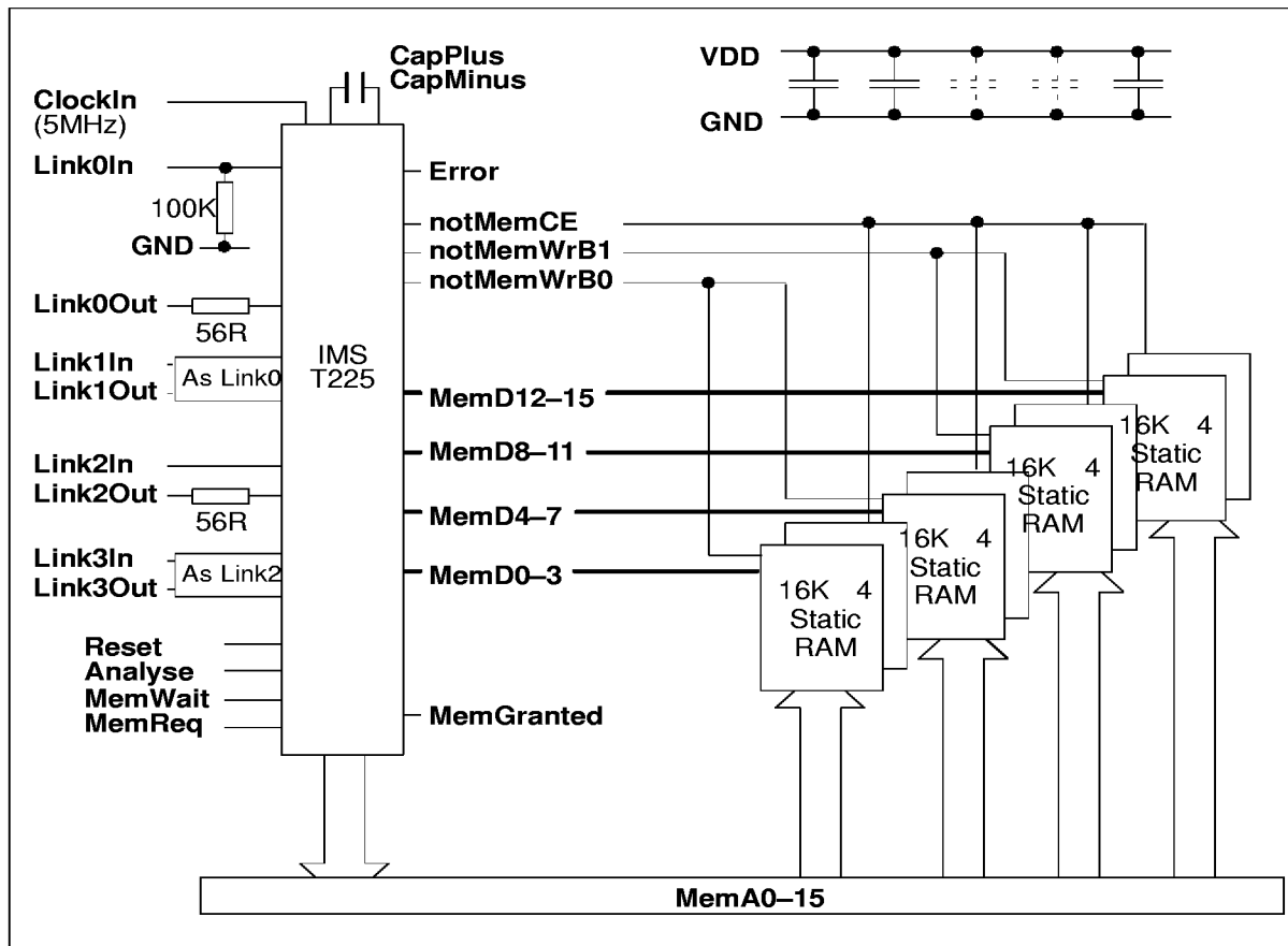
Figure 5.2 IMS T225E static RAM application
