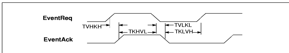
Figure 6.1 IMS T225E event timing
