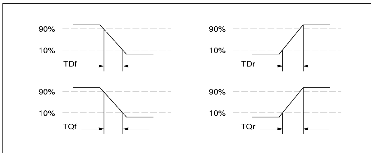
Figure 8.3 IMS T225E input and output edge timing
