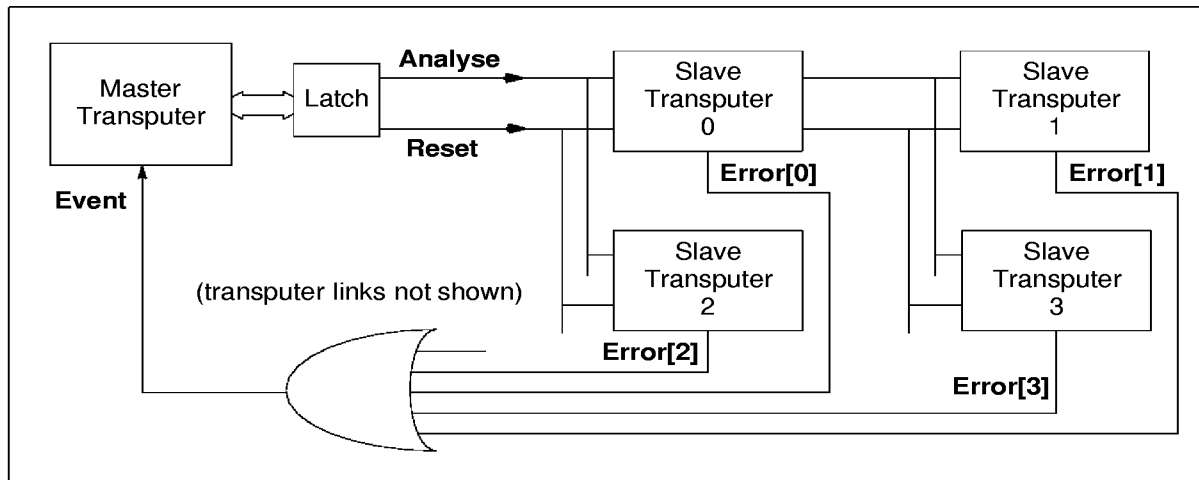
Figure 3.5 Error handling in a multi-transputer system
