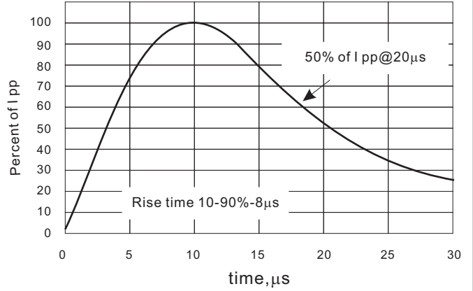
Pulse Waveform
