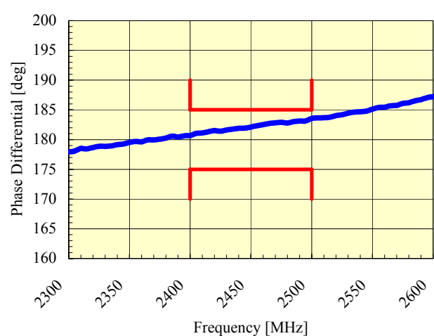
Phase Differential
