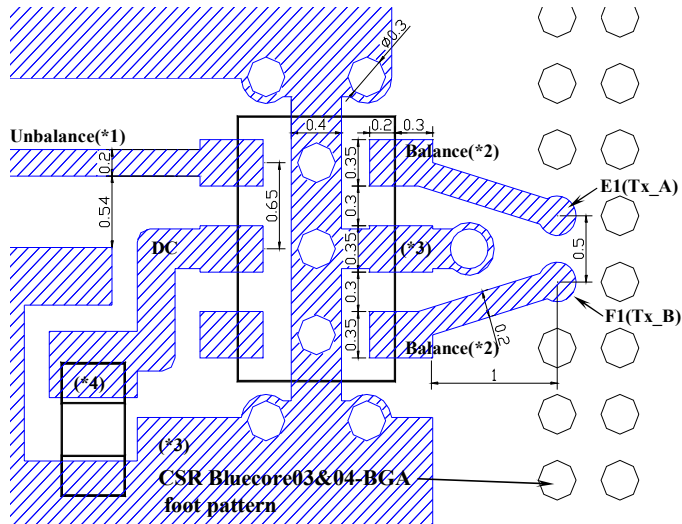
Land Pattern
