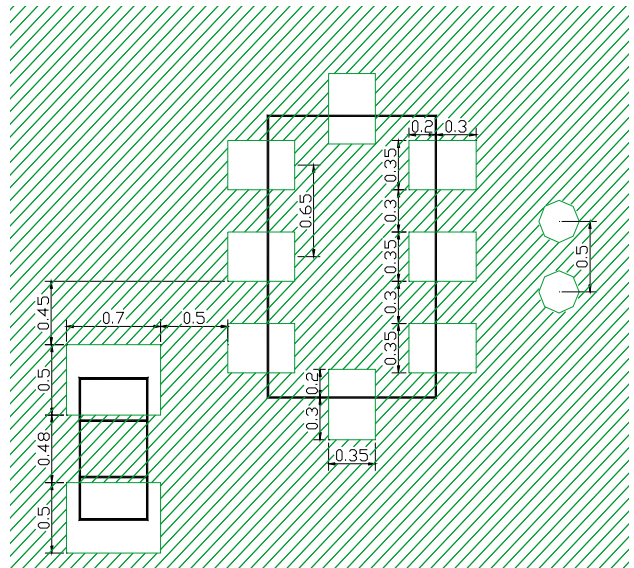
Resist Pattern
