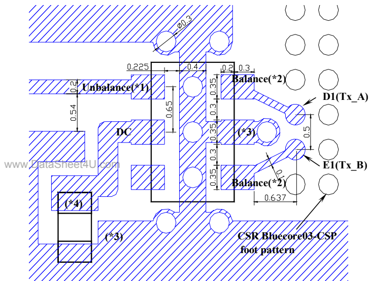
Land Pattern
