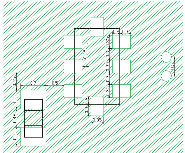
Resist Pattern
