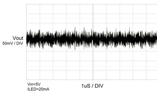
3S8P Output Ripple
