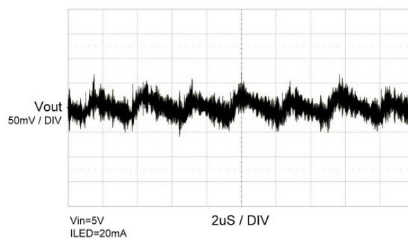
8S3P Output Ripple
