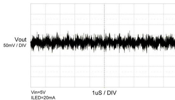
3S9P Output Ripple
