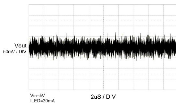
9S Output Ripple
