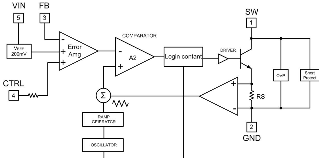
Figure 3: YB1520 Block Diagram
