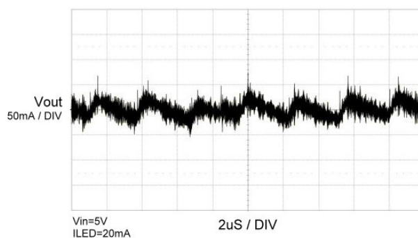
9S3P Output Ripple
