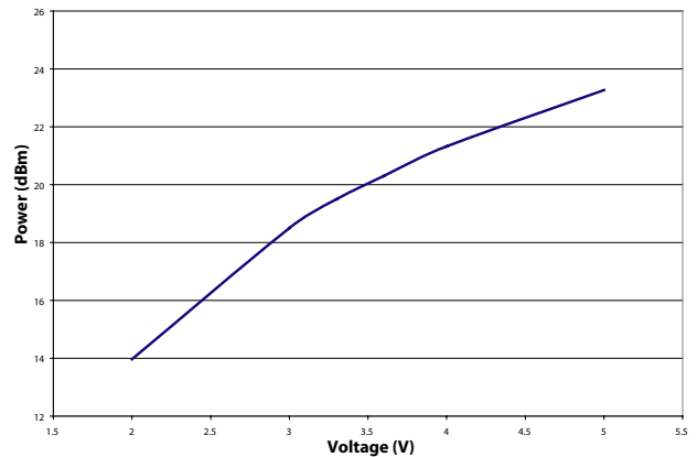
CCMM6004-SC Evaluation board @ 900MHz OIP3 Over Voltage
