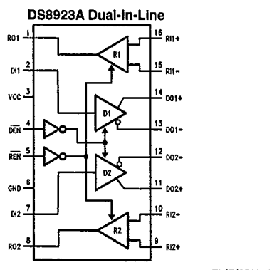
Order Number DS8923N, J, M DS8923AN, AJ, AM See NS Package Number N16A, J16A or M16A
