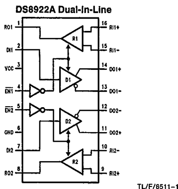
Order Number DS8922N, J, M, DS8922AN, AJ, AM See NS Package Number N16A, J16A or M16A
