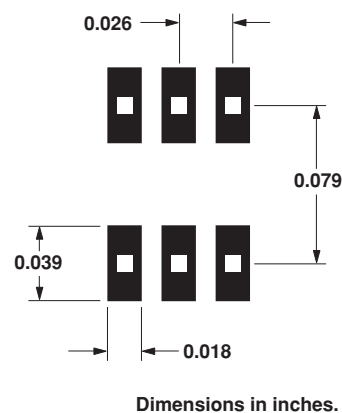
Figure 22. Recommended PCB Pad Layout for Agilent’s SC70 6L/SOT-363 Products.
