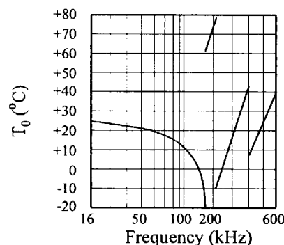
FIGURE 5. CX-2V Typical Turning Point Temperature ( T_0 )
