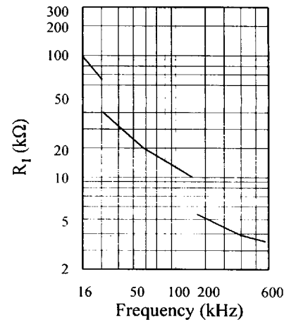
FIGURE 3. CX-2V Typical Motional Capacitance ( C_1 )
